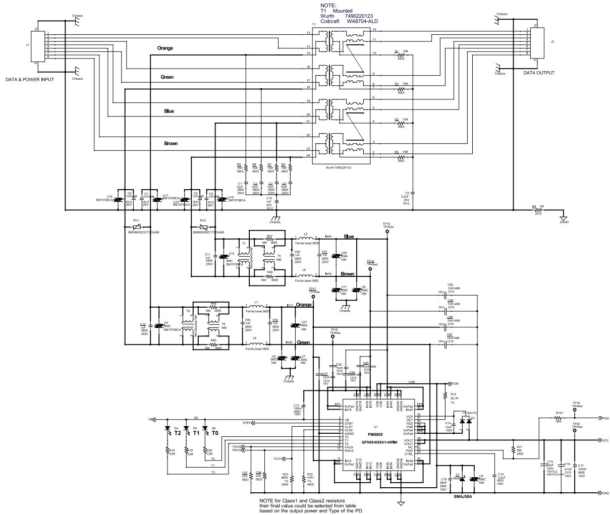
Figure 1: STEVAL-POE003V1 circuit schematic (1 of 3)
