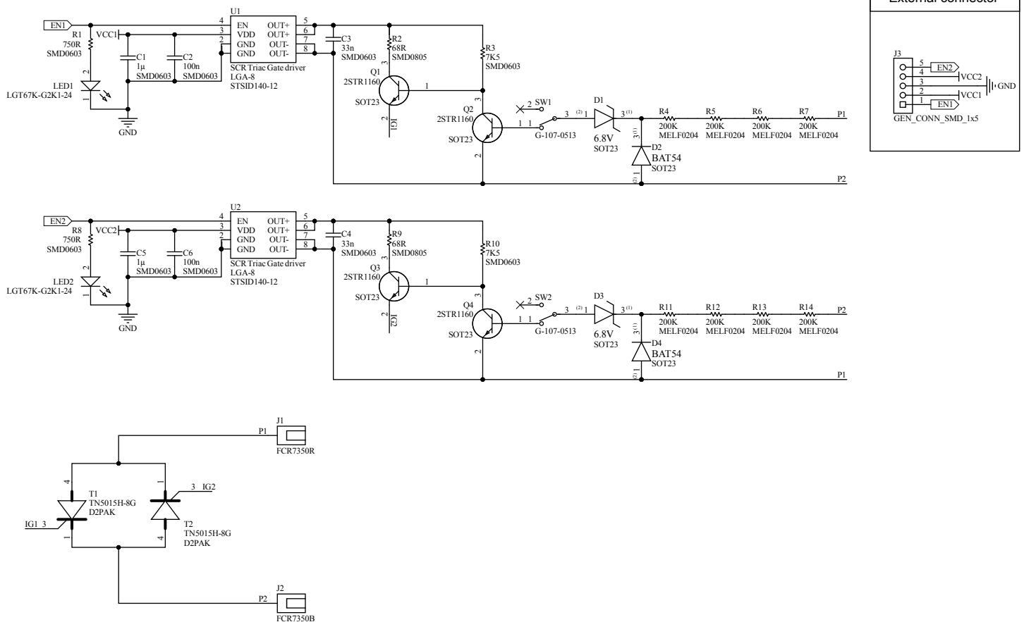
Figure 1. STEVAL-SID140V1 circuit schematic
