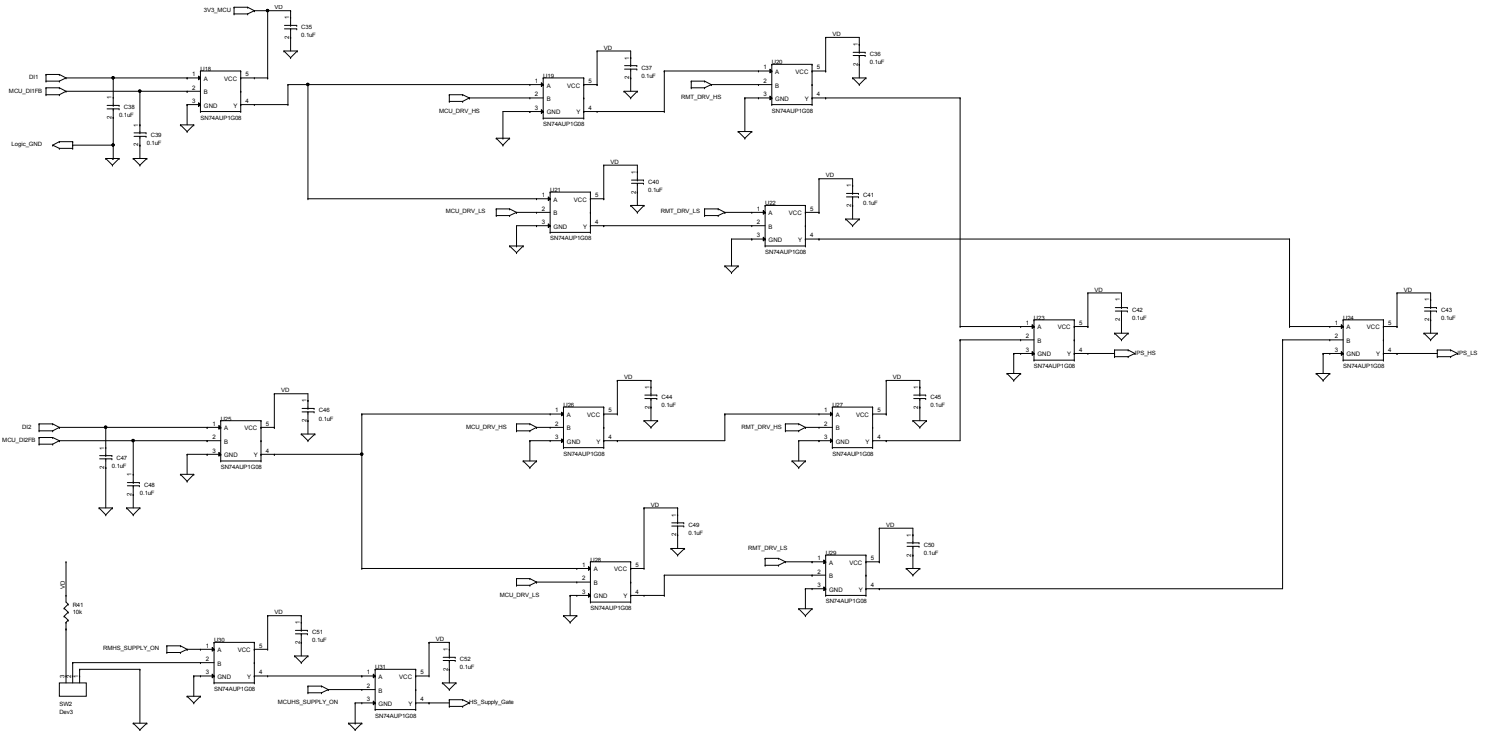
Figure 31. STEVAL-SILKTB01 circuit schematic (10 of 12)
