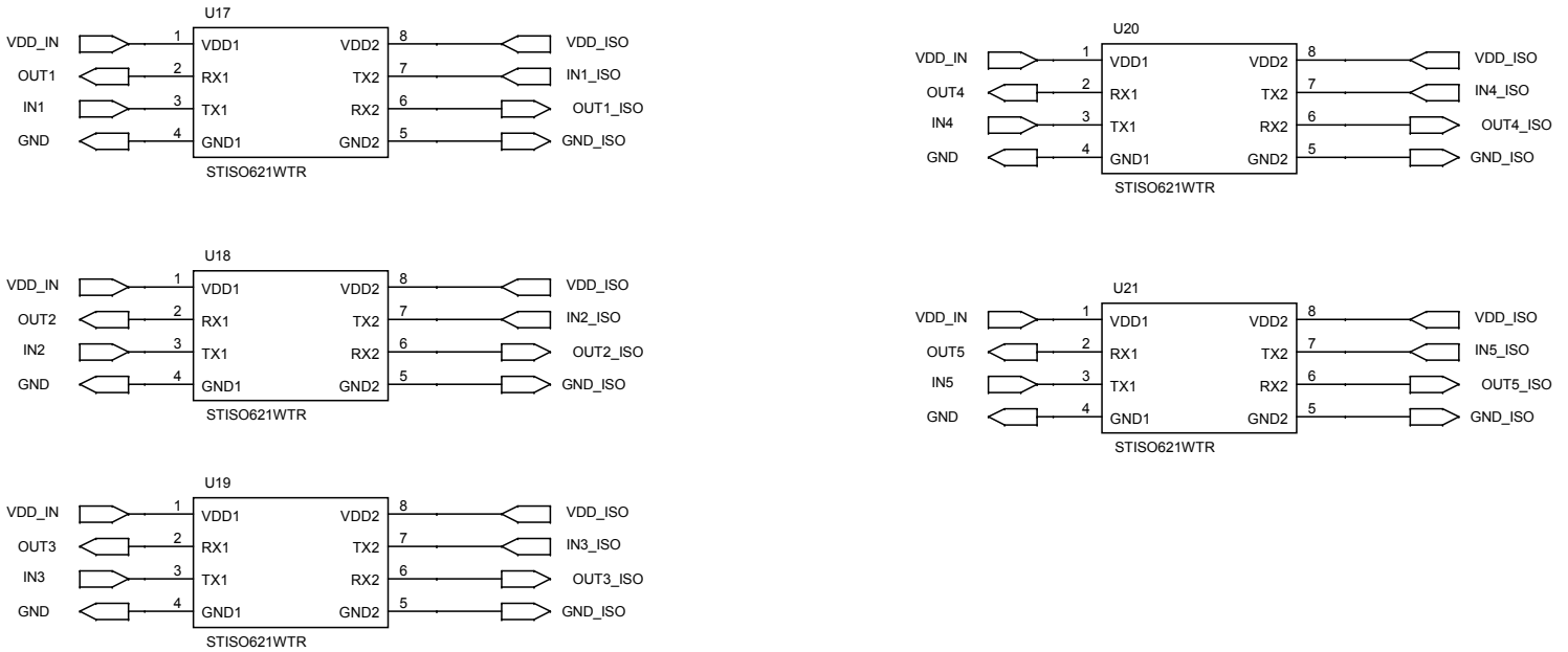
Figure 16. STEVAL-SILKTA01 circuit schematic (16 of 21)
