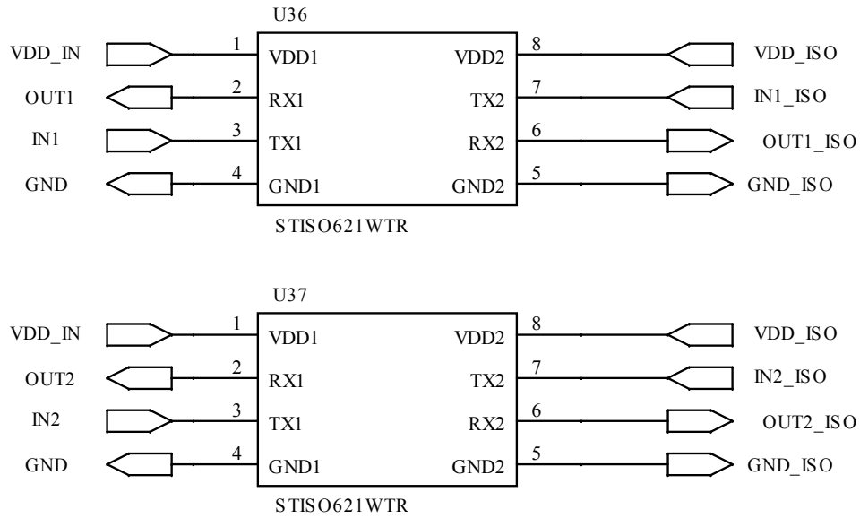
Figure 20. STEVAL-SILKTA01 circuit schematic (20 of 21)
