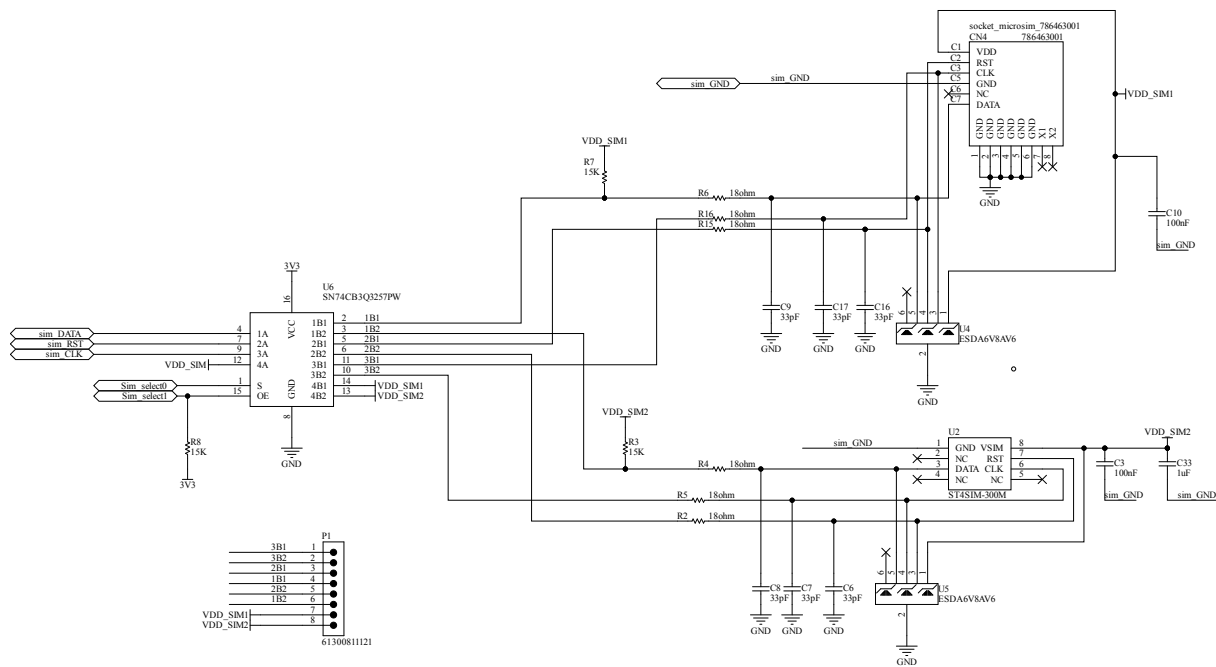
Figure 4. STEVAL-ST4SIMV1 circuit schematic (4 of 5)
