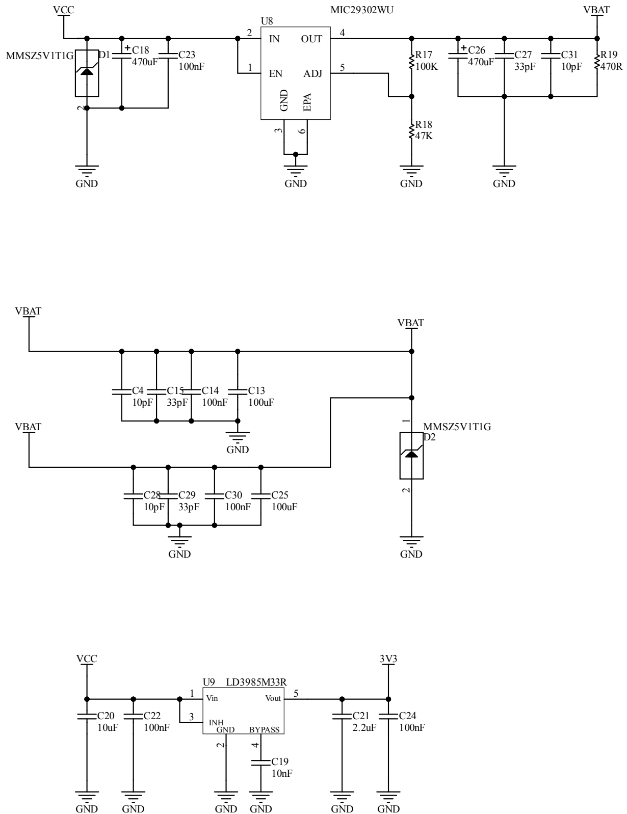
Figure 5. STEVAL-ST4SIMV1 circuit schematic (5 of 5)
