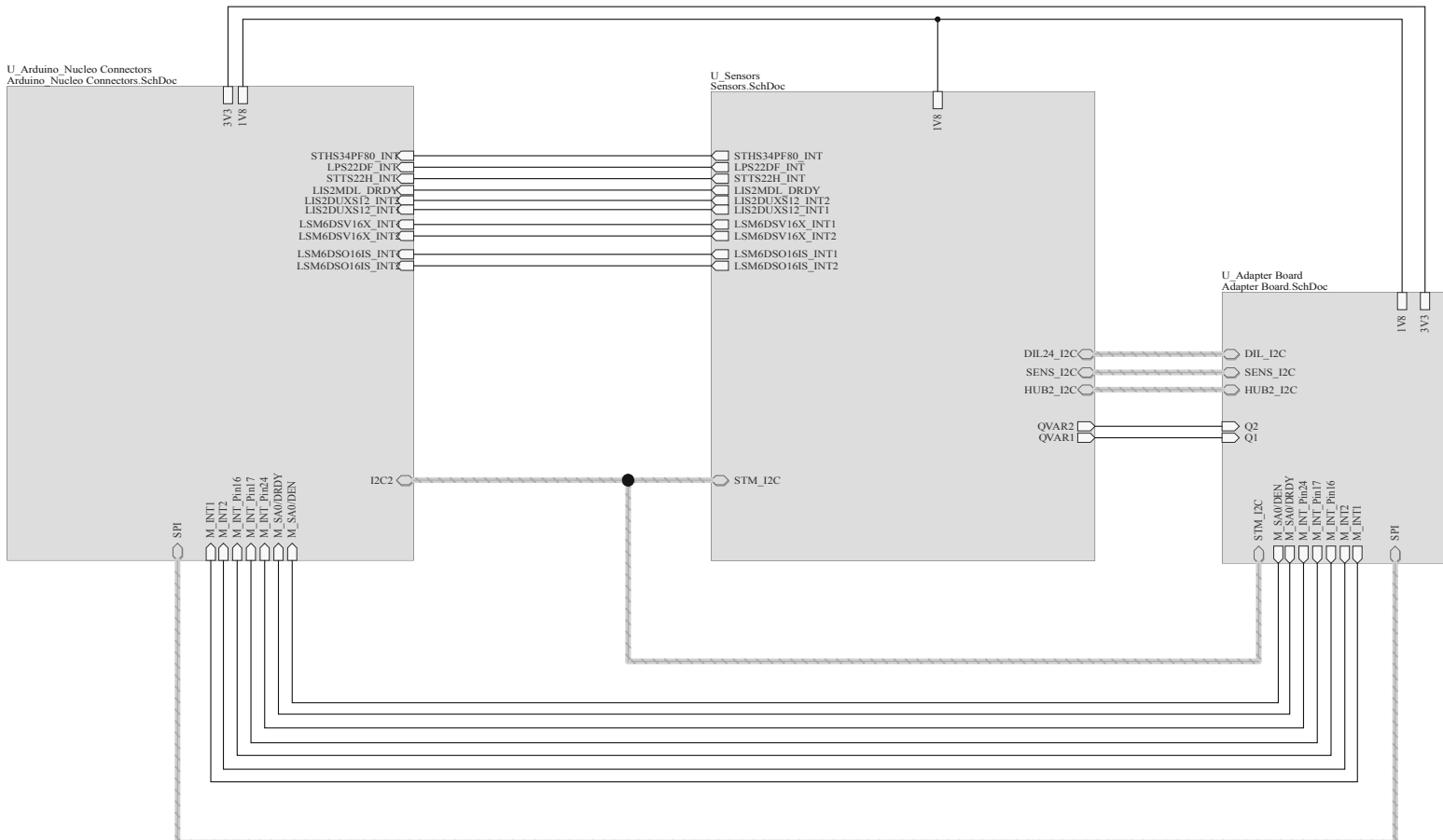
Figure 1. X-NUCLEO-IKS4A1 circuit schematic (1 of 4)
