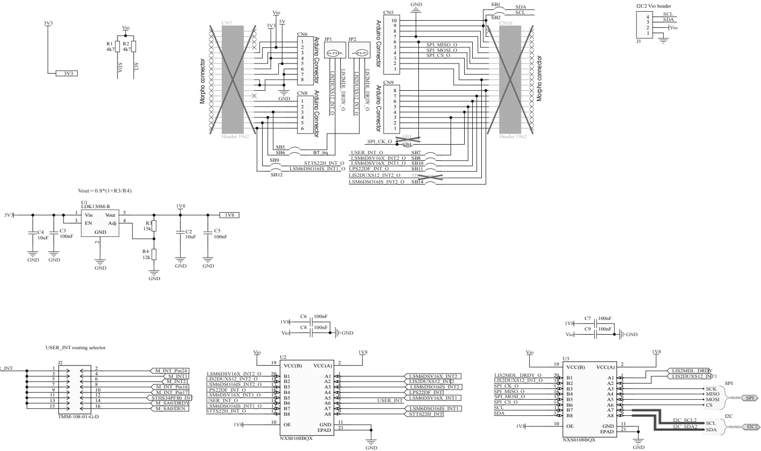
Figure 2. X-NUCLEO-IKS4A1 circuit schematic (2 of 4)
