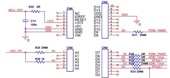
STM32 NUCLEO CONNECTORS (ARDUINO UNO R3)
