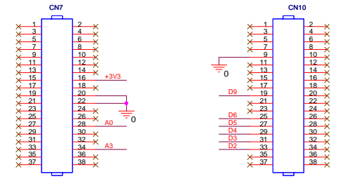
ST MORPHO CONNECTORS
