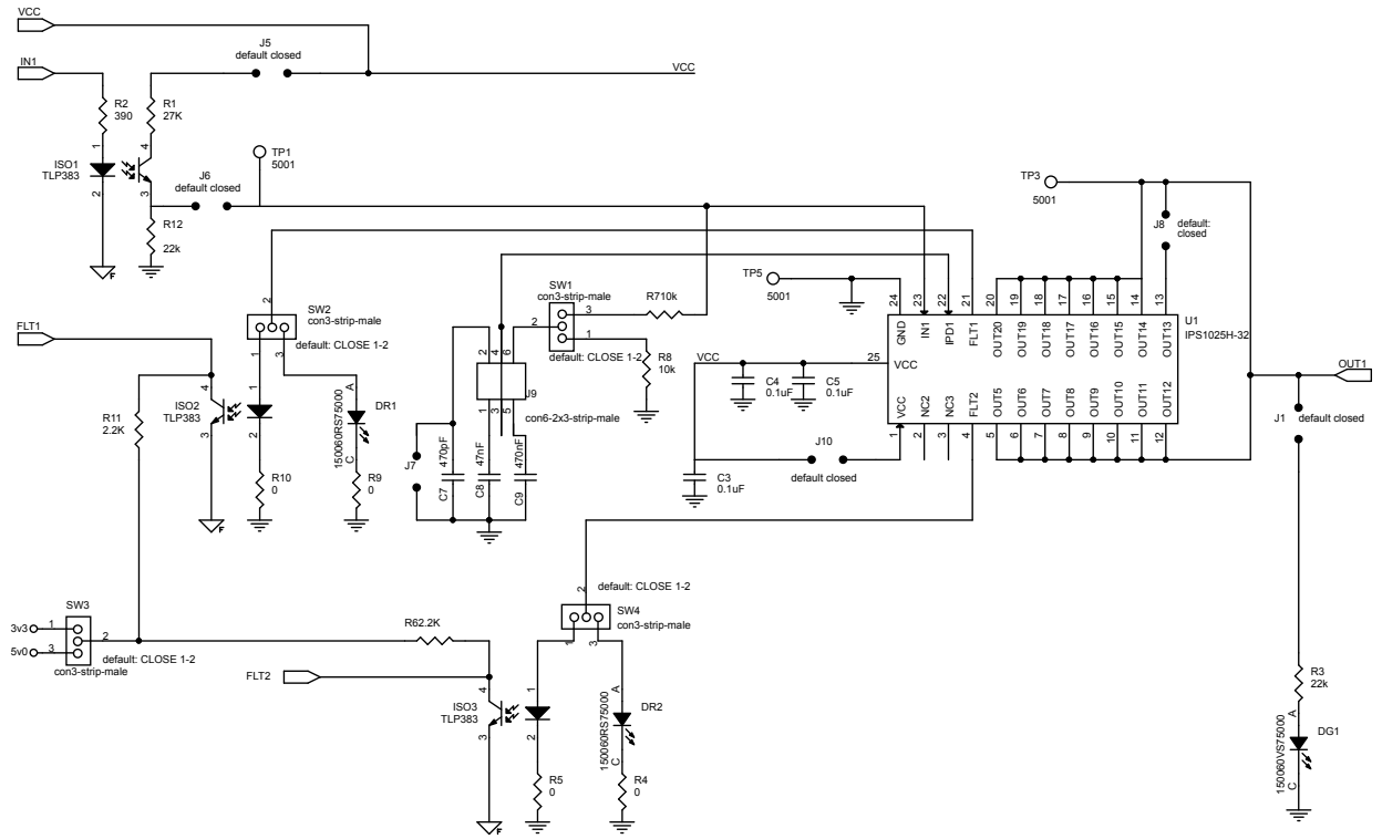
Figure 2. X-NUCLEO-OUT06A1 circuit schematic (2 of 2)
