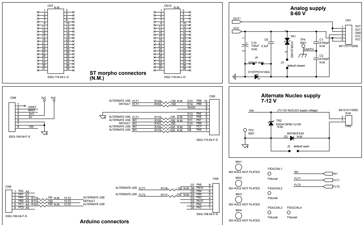
Figure 1. X-NUCLEO-OUT06A1 circuit schematic (1 of 2)
