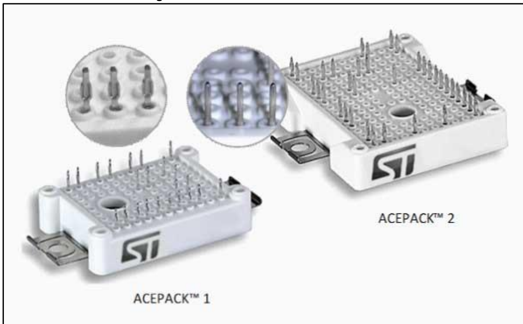
Figure 1: ACEPACK™ 1 and ACEPACK™ 2
