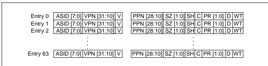
Figure 9: UTLB configuration
