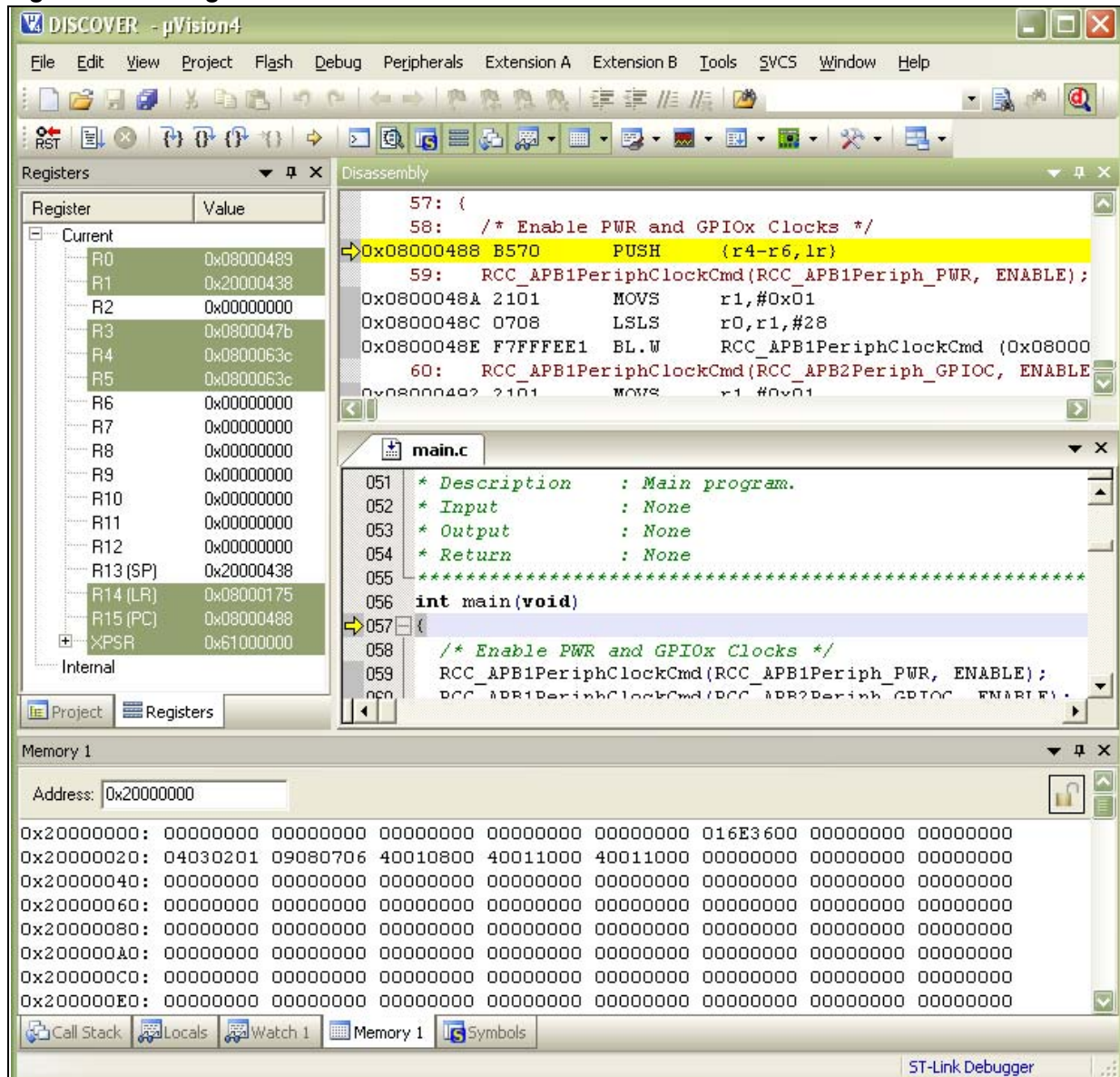
Figure 11. Debug screens
