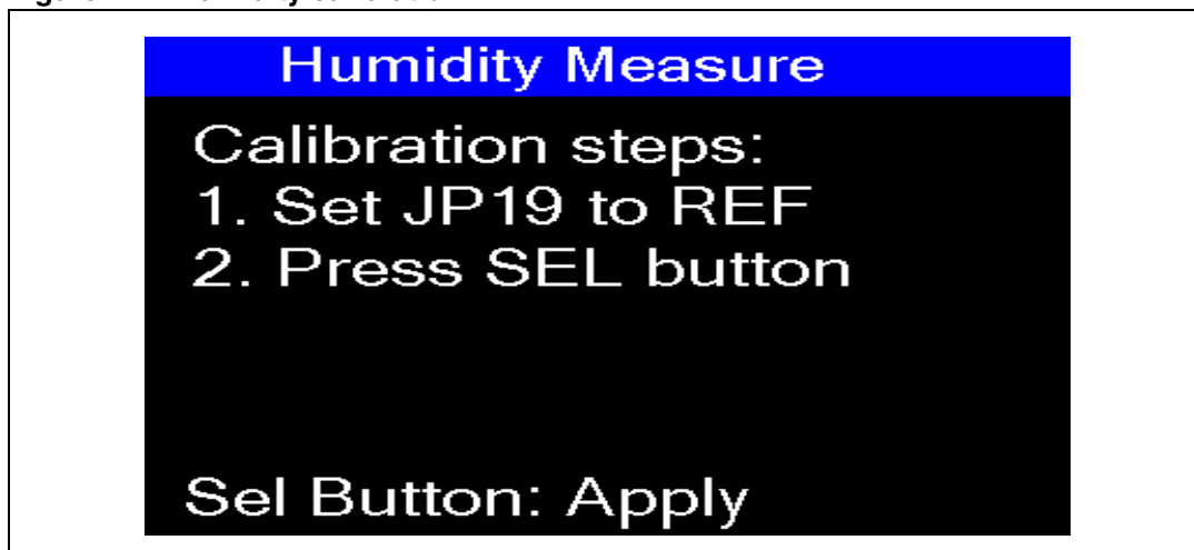
Figure 72. Humidity calibration 1
