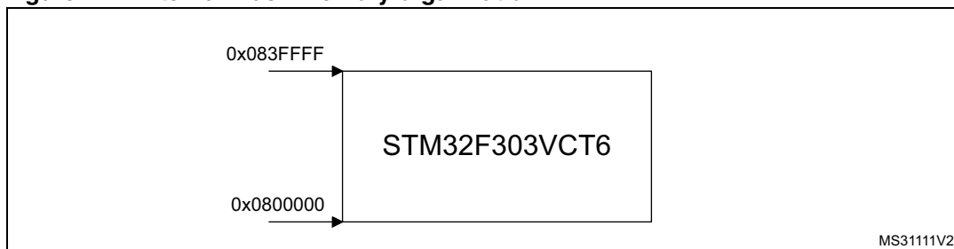
Figure 14. Internal Flash memory organization
