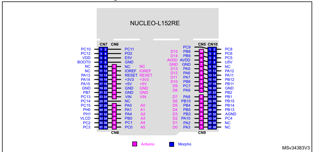
Figure 21. NUCLEO-L152RE
