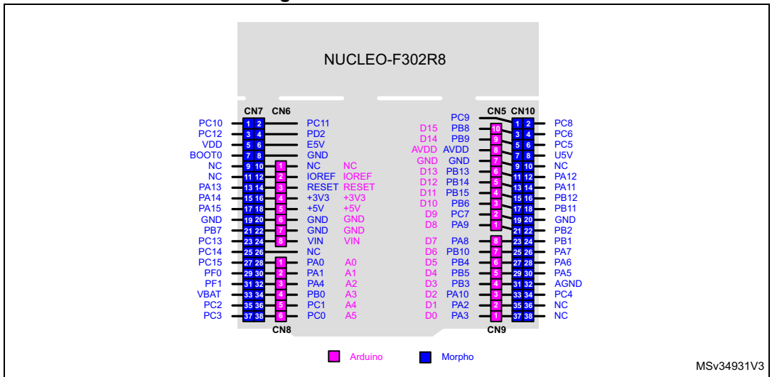
Figure 14. NUCLEO-F302R8
