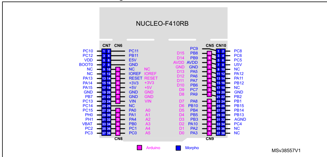
Figure 25. NUCLEO-F410RB
