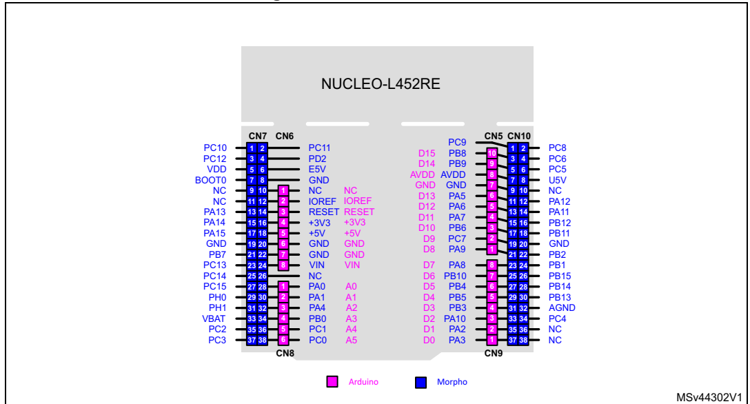
Figure 22. NUCLEO-L452RE
