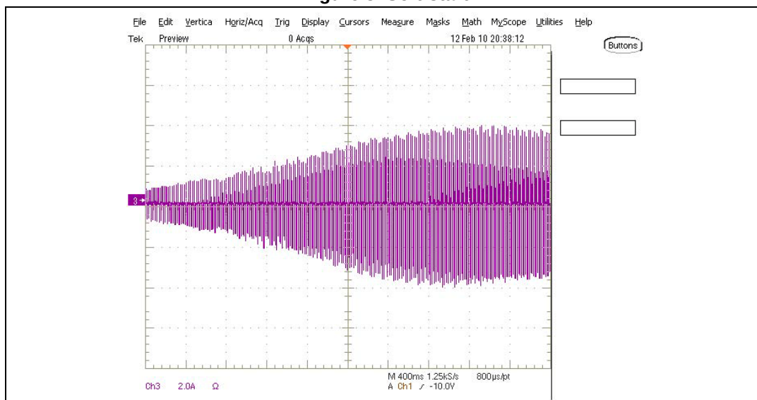
Figure 8. Soft-start
