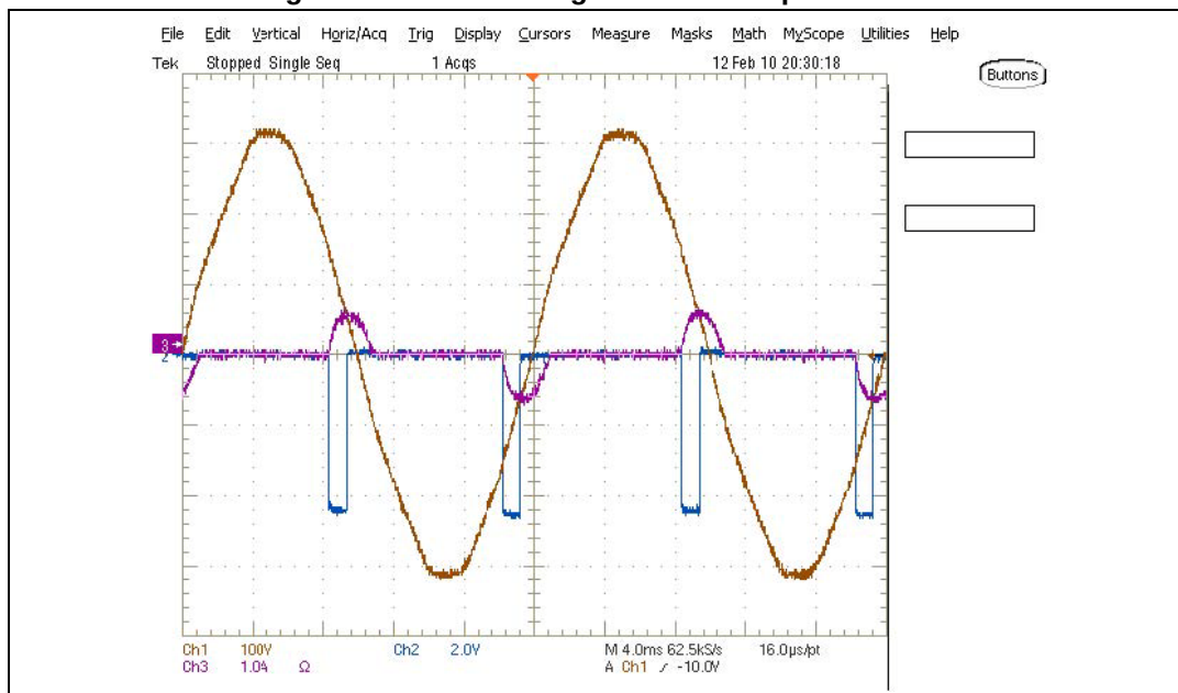
Figure 5. Motor running at the lowest power level
