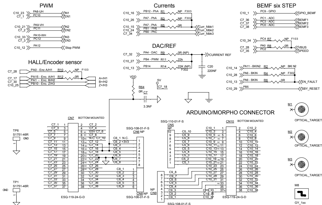
Figure 3. X-NUCLEO-IHM17M1 circuit schematic (1 of 2)
