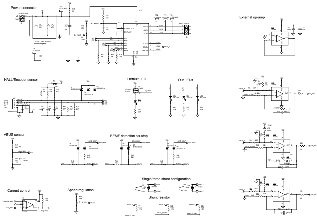
Figure 4. X-NUCLEO-IHM17M1 circuit schematic (2 of 2)
