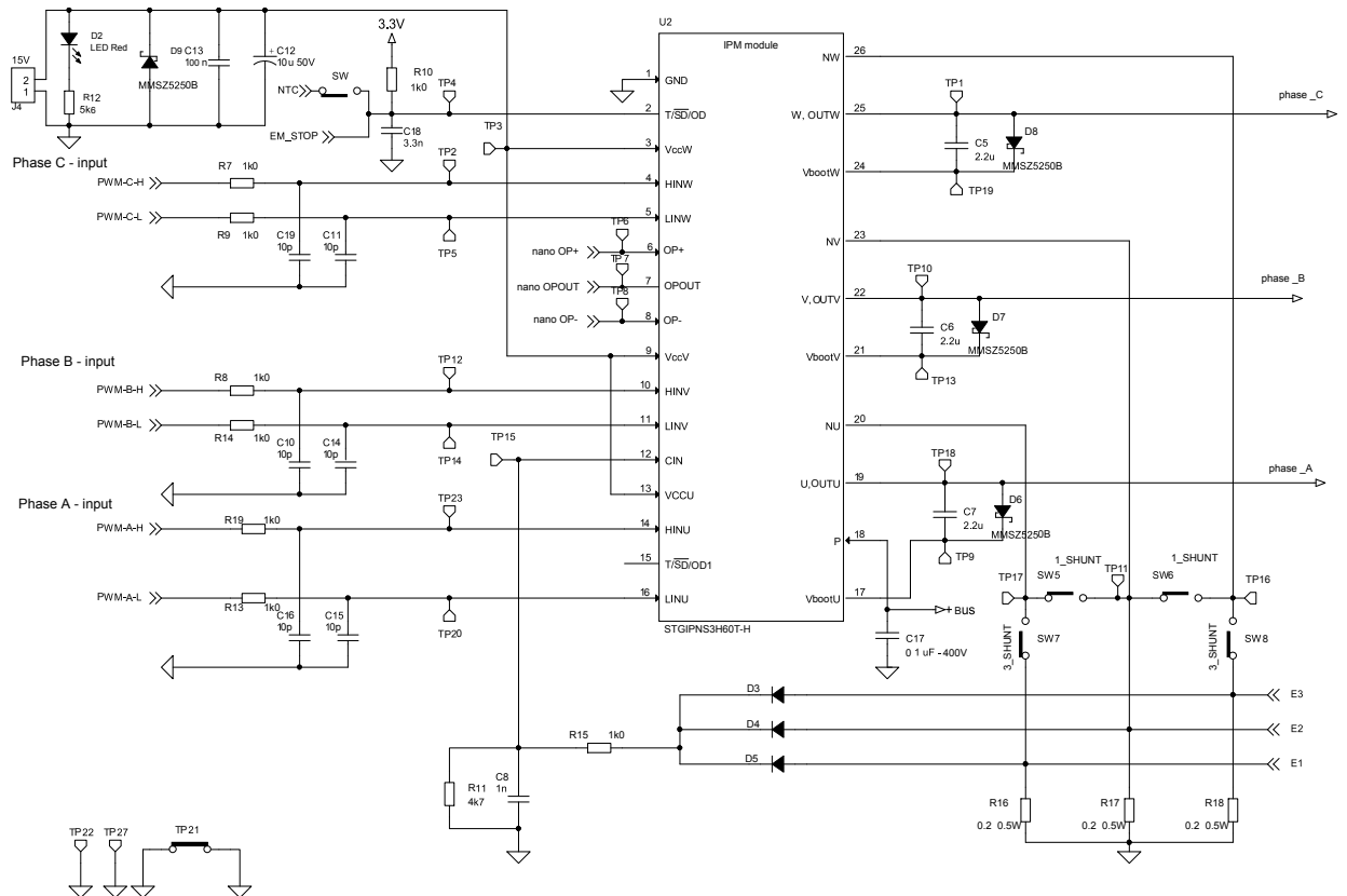
Figure 4. STEVAL-IPMnG3S - circuit schematic (3 of 5)
