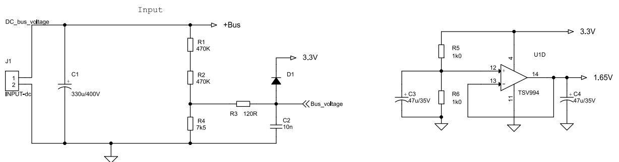
Figure 2. STEVAL-IPMnG3S - circuit schematic (1 of 5)
