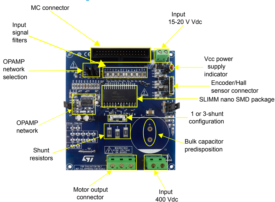
Figure 7. STEVAL-IPMnG3S architecture
