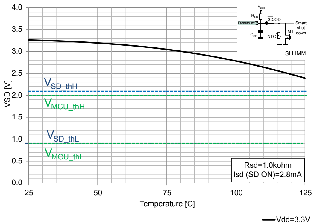
Figure 11. NTC voltage vs temperature
