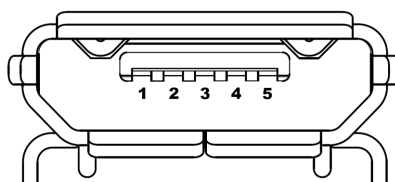
Figure 10. USB Micro-B connector (CN14) front view
