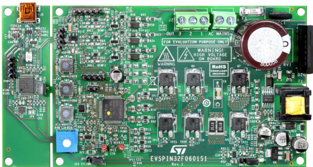
Figure 1. EVSPIN32F0601S1 - Evaluation board
