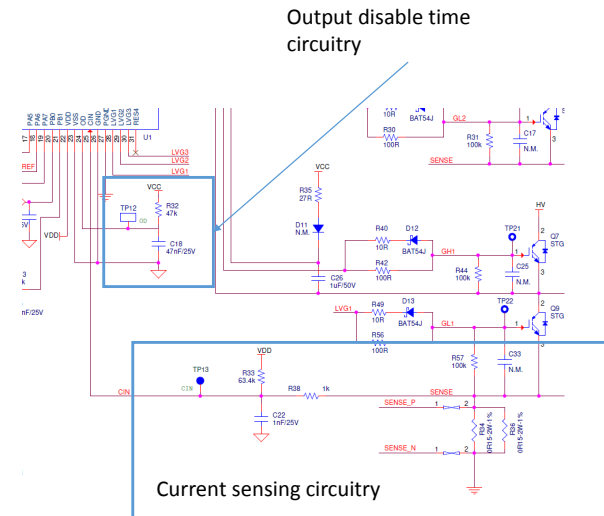
Figure 4. EVSPIN32F0601S1 - Current sensing and disable time circuitry
