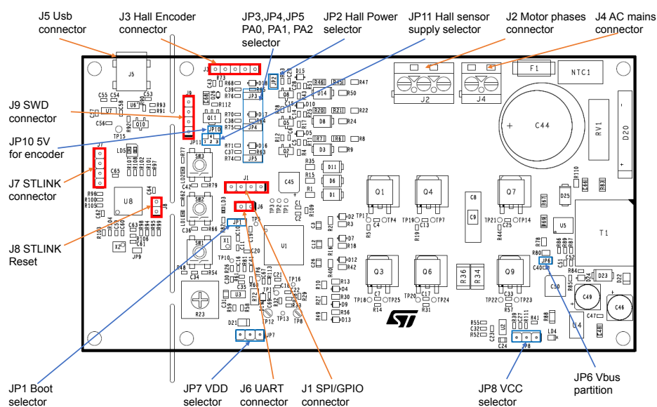
Figure 3. EVSPIN32F0601S1 - Main components and connectors position
