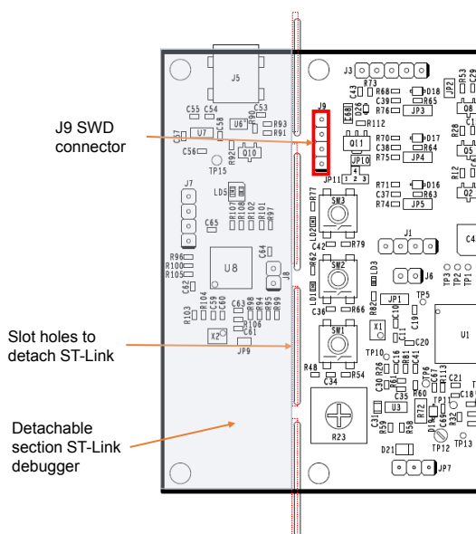
Figure 5. EVSPIN32F0601S1 - Detachable section
