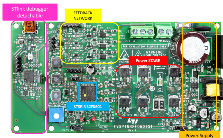
Figure 2. EVSPIN32F0601S1 - Board functions description
