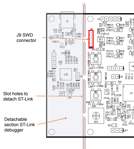
Figure 5. EVSPIN32F0602S1 - Detachable section
