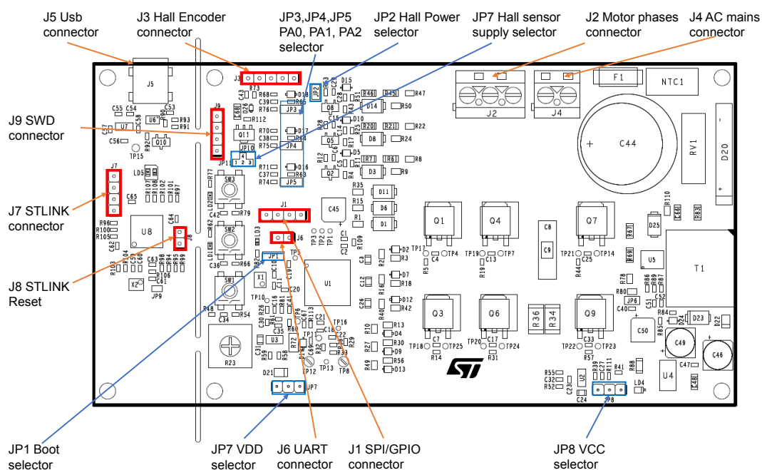
Figure 3. EVSPIN32F0602S1 – Main components and connectors position
