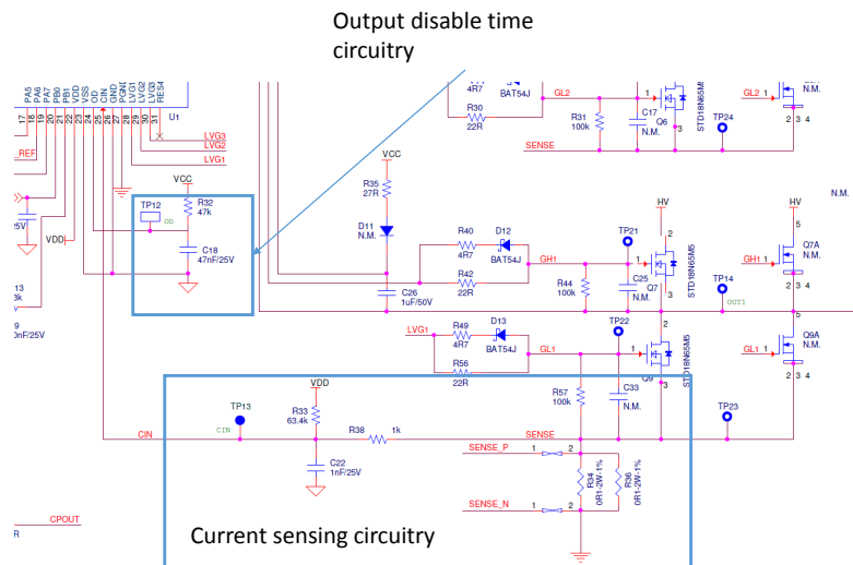
Figure 4. EVSPIN32F0602S1 - Current sensing and disable time circuitry
