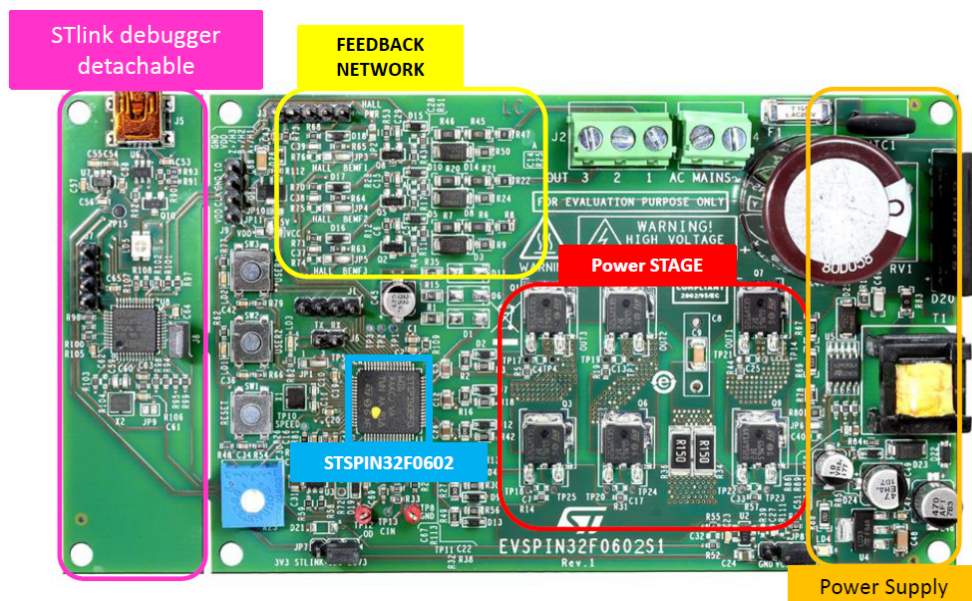
Figure 2. EVSPIN32F0602S1 – board function description
