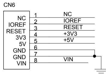
Figure 5. X-NUCLEO-BNRG2A1 schematic diagram - Arduino connectors
