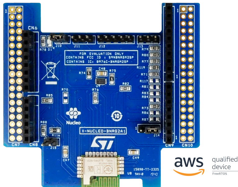
Figure 1. X-NUCLEO-BNRRG2A1 expansion board
