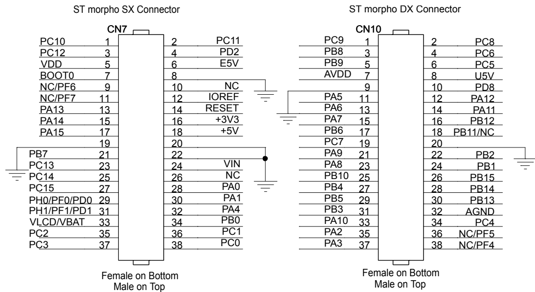
Figure 6. X-NUCLEO-BNRG2A1 schematic diagram - morpho connectors
