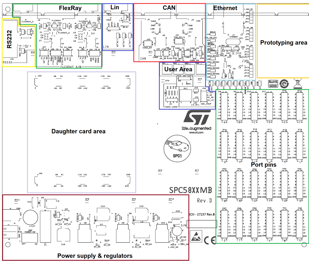
Figure 3. EVB functional blocks
