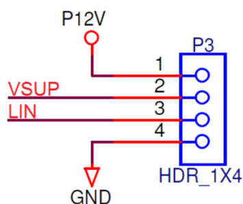
Figure 10. LIN 4pin header interface connector
