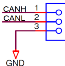
Figure 7. CAN 3pin header interface connector
