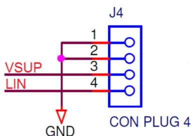
Figure 9. LIN molex connector
