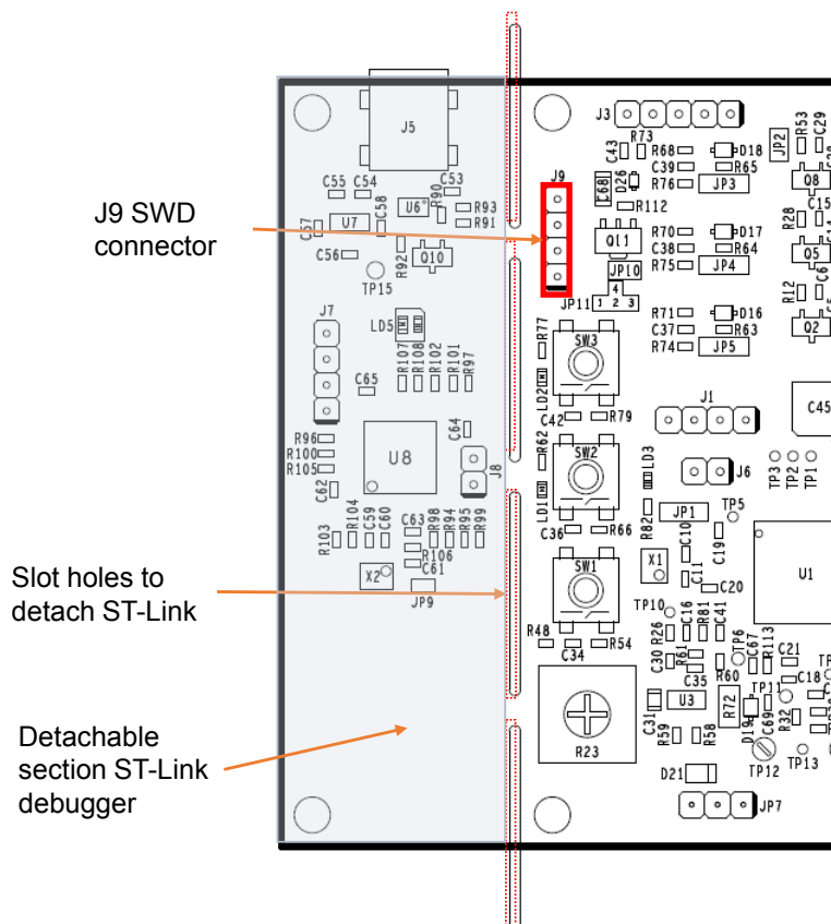
Figure 5. EVSPIN32F06Q2S1 - detachable section
