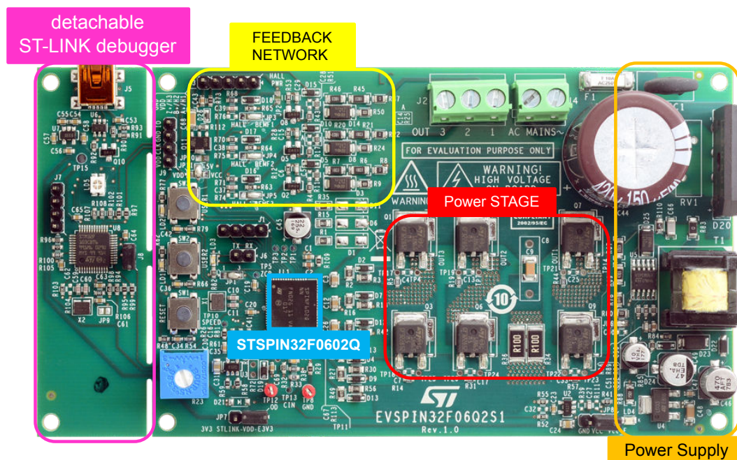
Figure 2. EVSPIN32F06Q2S1 - Board functions
