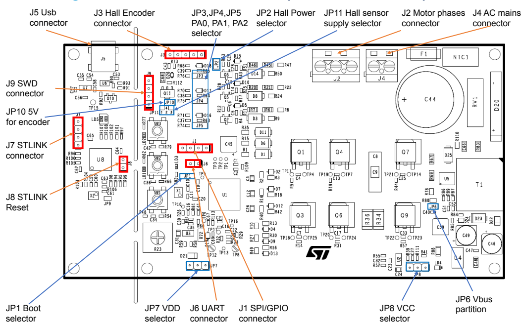
Figure 3. EVSPIN32F06Q2S1 - Main components and connector positions
