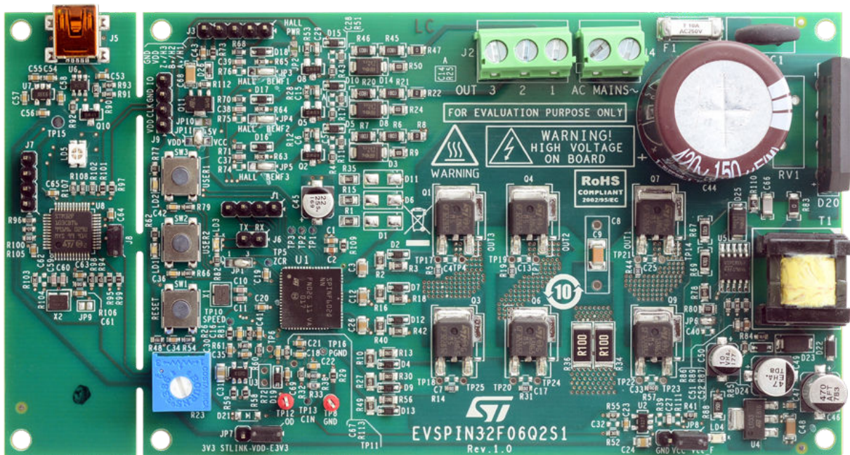
Figure 1. EVSPIN32F06Q2S1 evaluation board
