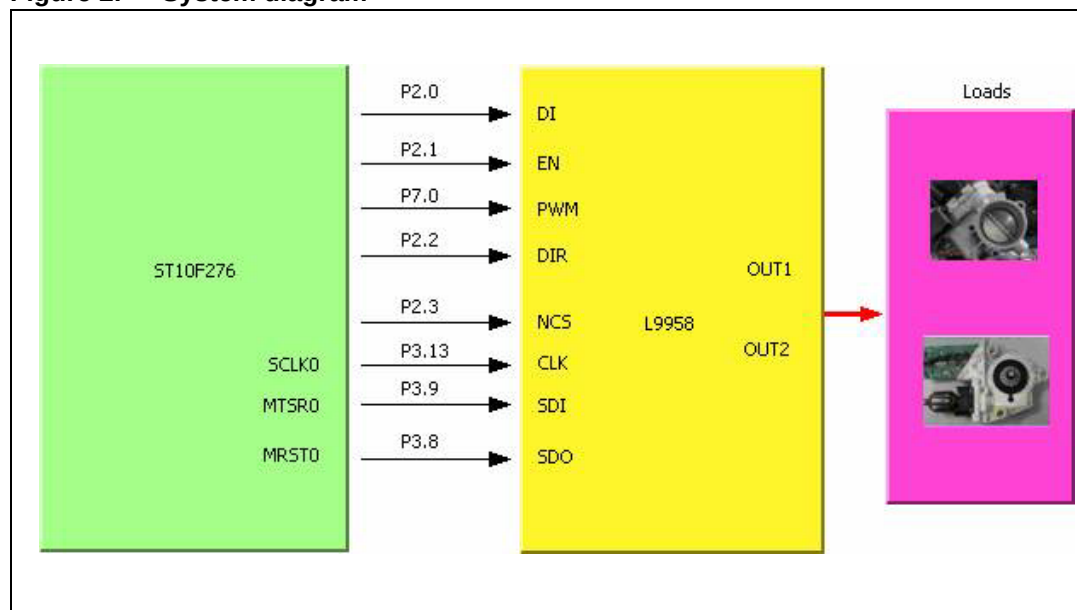
Figure 2. System diagram
