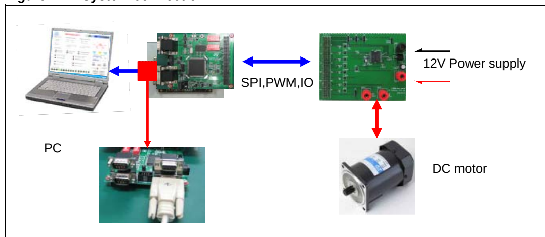
Figure 2. System diagram
