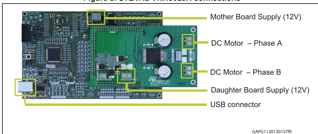
Figure 3. STEVAL-VNH5019A connections
