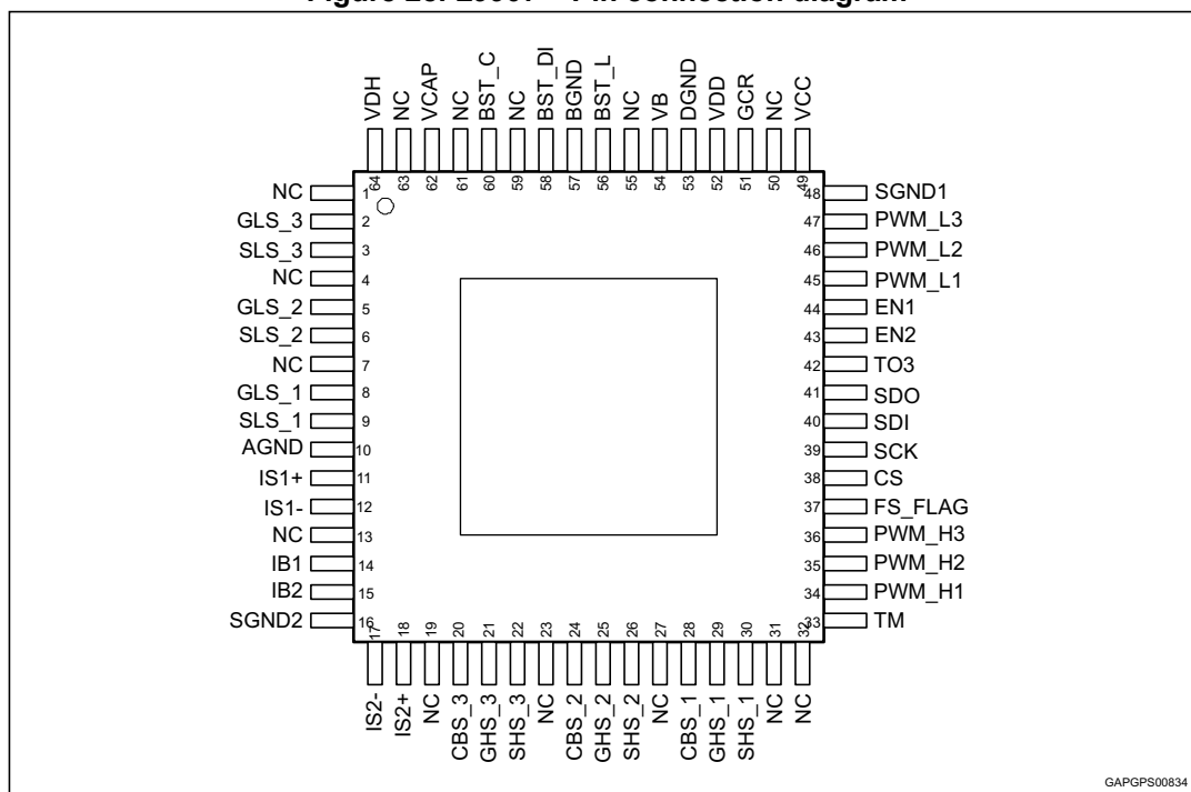
Figure 28. L9907 – Pin connection diagram
