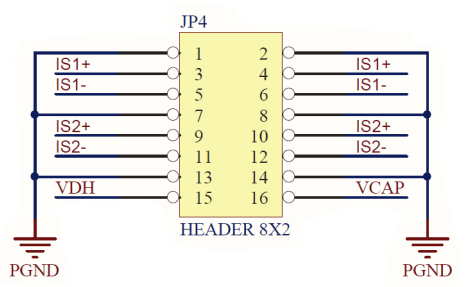
Figure 16. Inverter board connector - phase signals- Female
