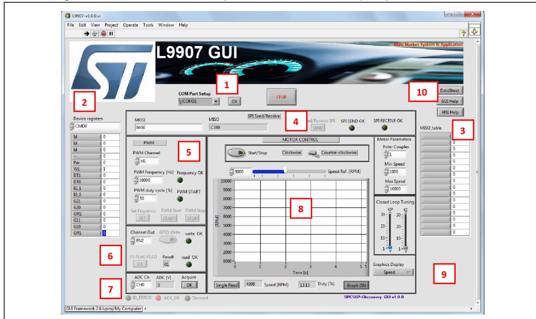
Figure 17. STSW-L9907 Graphical User Interface (GUI) for EVAL-L9907
