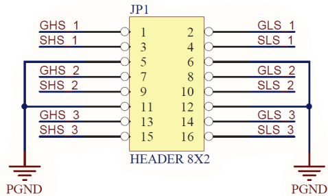
Figure 13. Inverter board connector - control signals- Male
