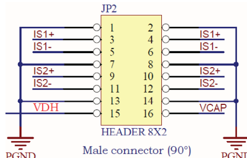
Figure 12. Gate driver board connector: phase signals
