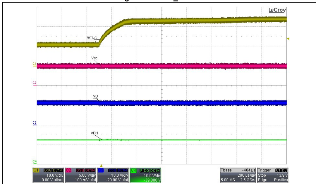
Figure 18. Vbst_c Start
