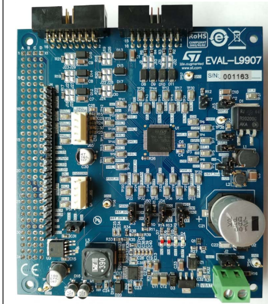
Figure 2. Gate driver board - top view
