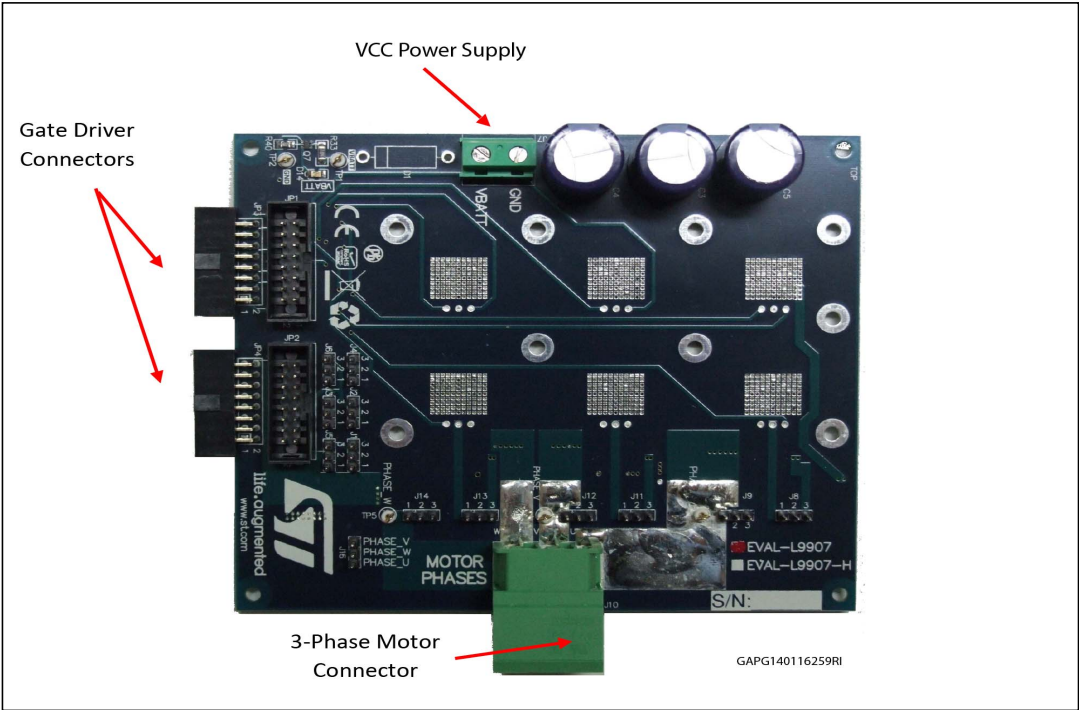
Figure 8. Output Power Board - Components and connectors (Top view)
