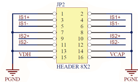
Figure 15. Inverter board connector - phase signals- Male
