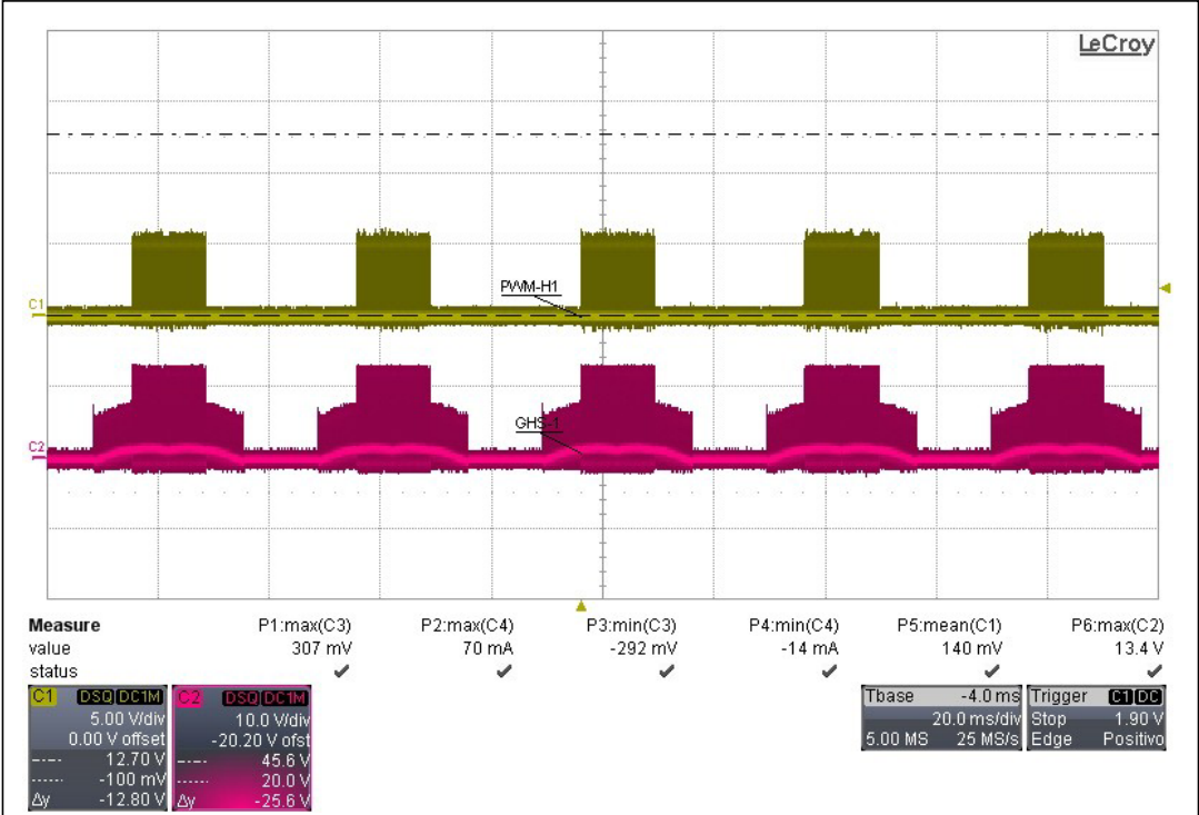
Figure 19. BLDC motor running PWM_H1/GHS_1
