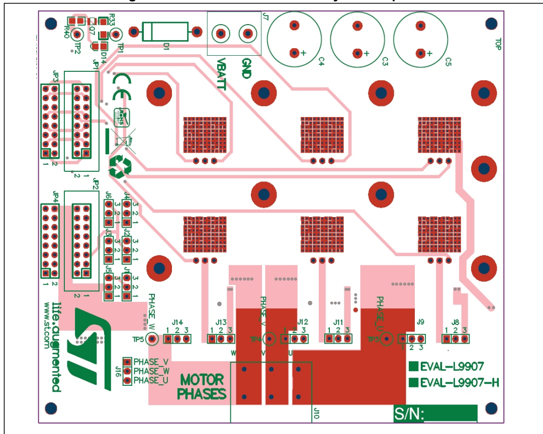
Figure 34. Inverter board - PCB Layout – Top view
