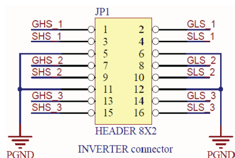
Figure 11. Gate driver board connector: control signals
