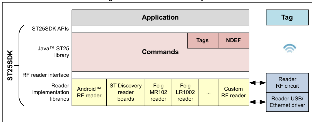
Figure 5. ST25SDK software layers
