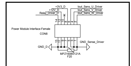
Figure 24. STEVAL-CTM001V1D circuit schematic (2 of 6)
