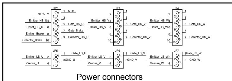
Figure 24. STEVAL-CTM001V1D circuit schematic (2 of 6)
