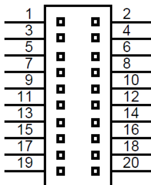
Figure 18. STEVAL-CTM001V1: JTAG connector (CON14)
