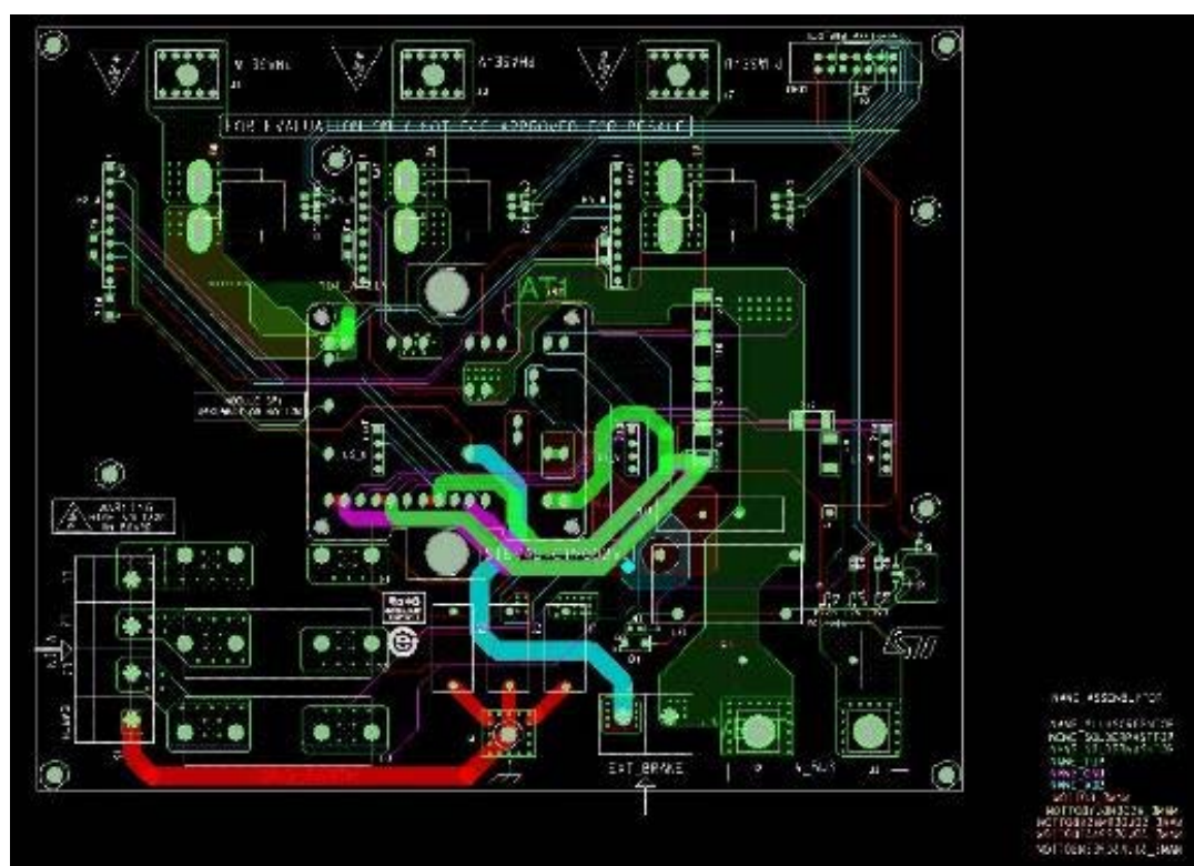
Figure 19. STEVAL-CTM002V1 layout
