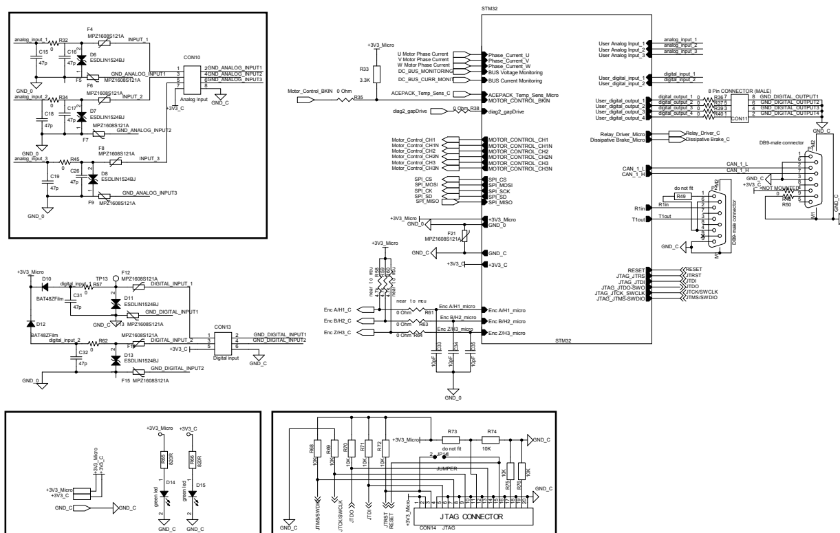
Figure 30. STEVAL-CTM001V1C circuit schematic (2 of 3)
