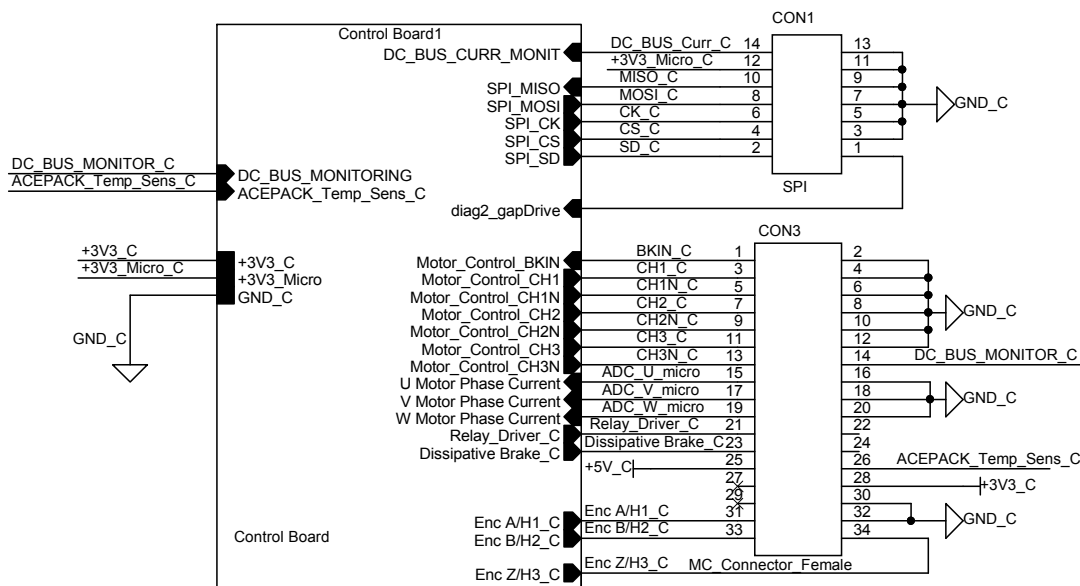
Figure 30. STEVAL-CTM001V1C circuit schematic (2 of 3)
