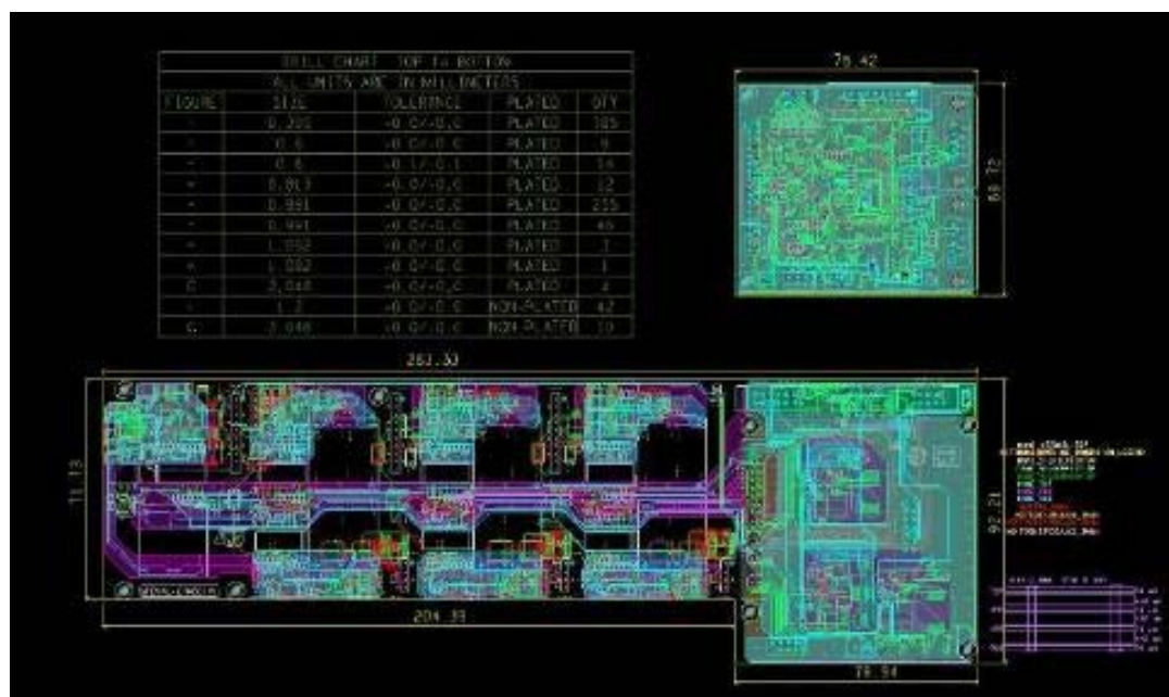
Figure 20. STEVAL-CTM001V1 layout
