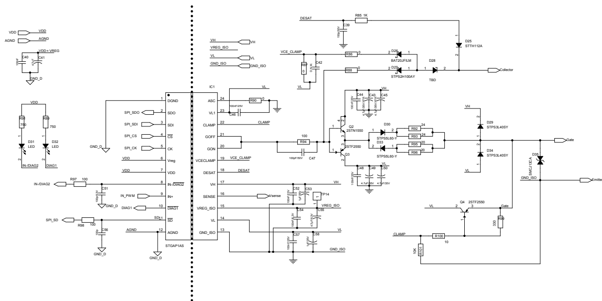
Figure 26. STEVAL-CTM001V1D circuit schematic (4 of 6)
