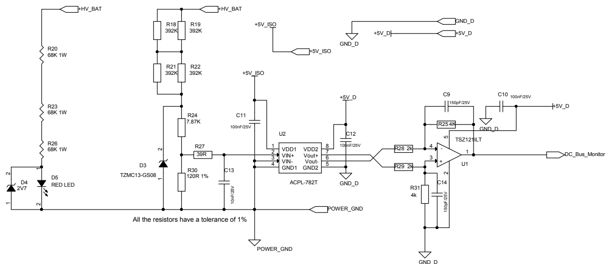
Figure 24. STEVAL-CTM001V1D circuit schematic (2 of 6)
