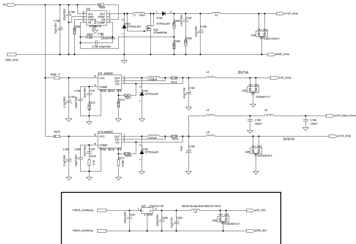
Figure 28. STEVAL-CTM001V1D circuit schematic (6 of 6)
