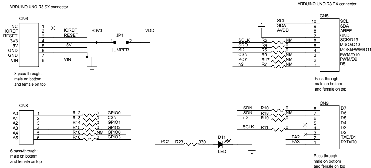
Figure 5. X-NUCLEO-S2915A1 circuit schematic - Arduino connectors
