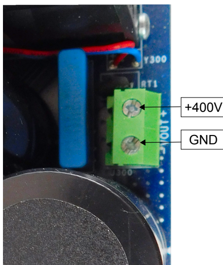
Figure 4. STEVAL-IPFC02P1 DC output connection
