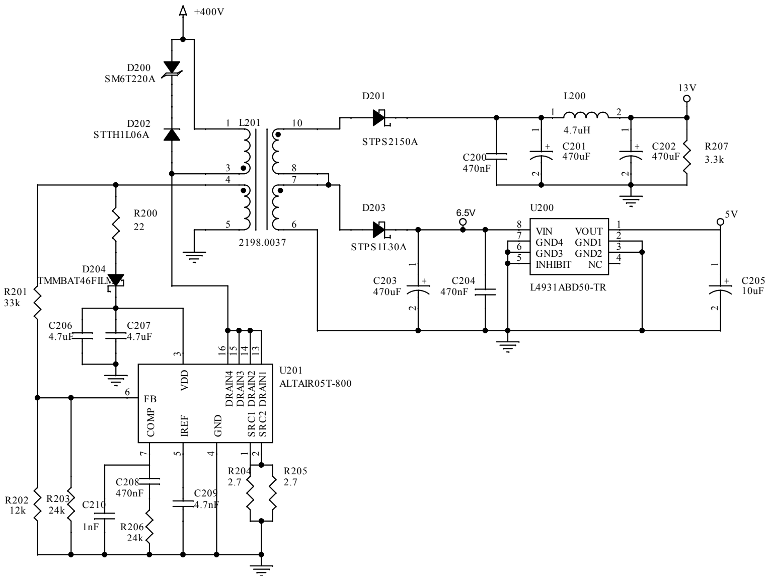
Figure 8. STEVAL-IPFC02P1 schematic - auxiliary power supply
