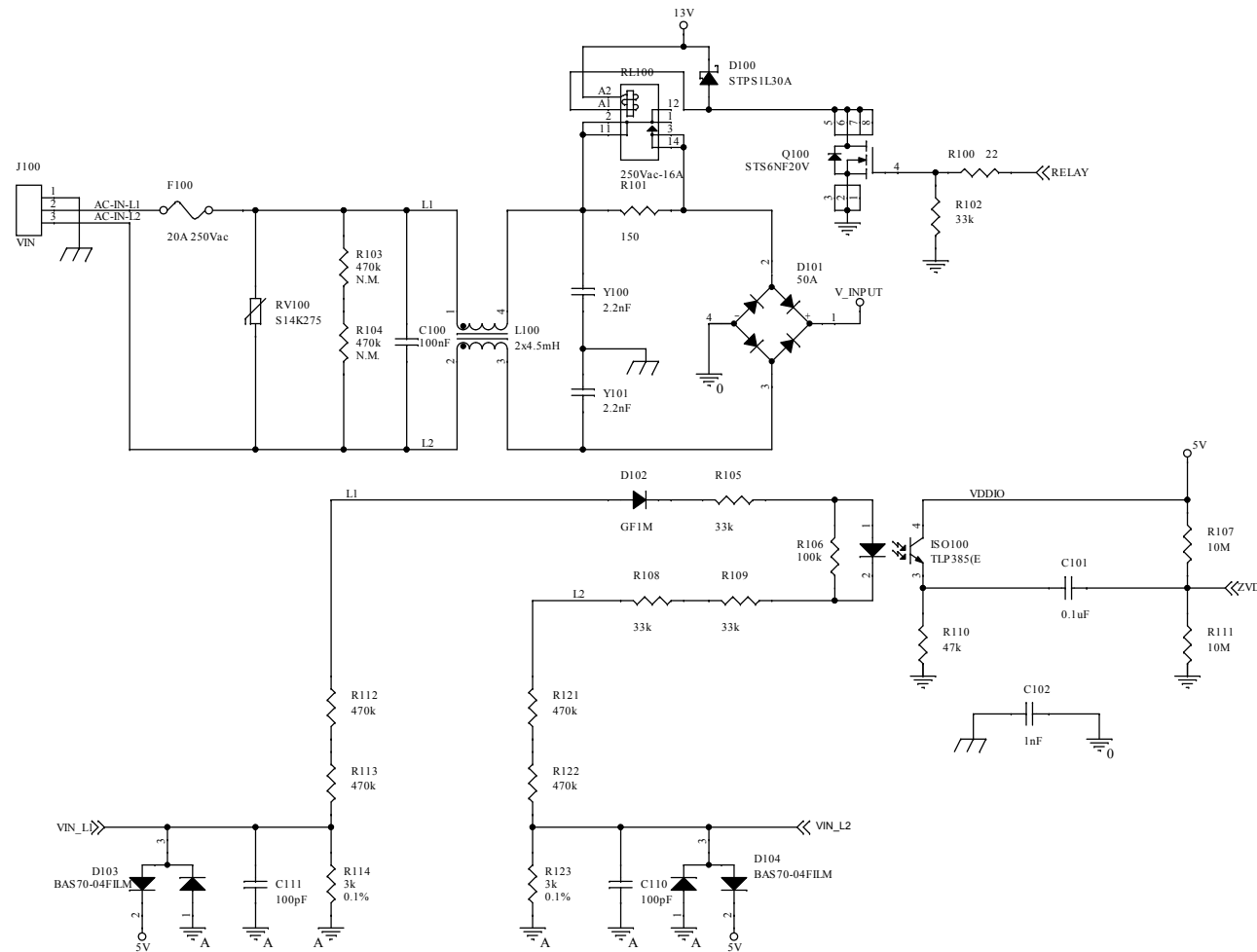
Figure 7. STEVAL-IPFC02P1 schematic - input section
