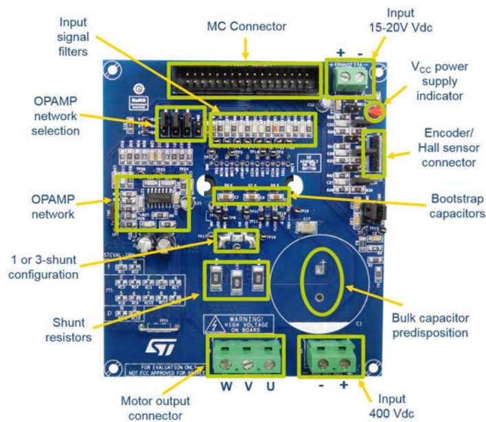
Figure 8. STEVAL-IPMNM3Q architecture
