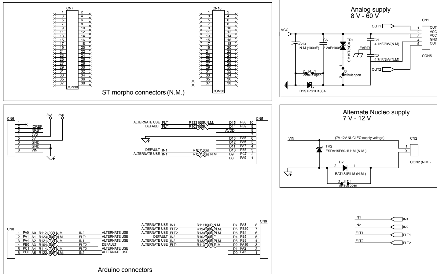
Figure 5. X-NUCLEO-OUT03A1 circuit schematic (1 of 2)
