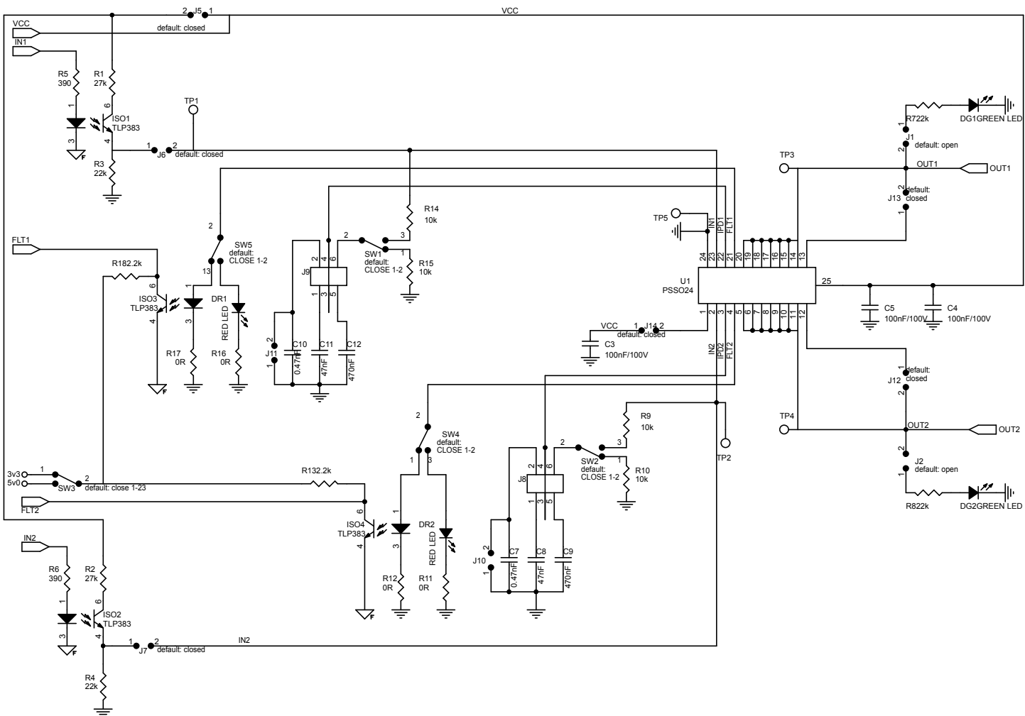
Figure 6. X-NUCLEO-OUT03A1 circuit schematic (2 of 2)
