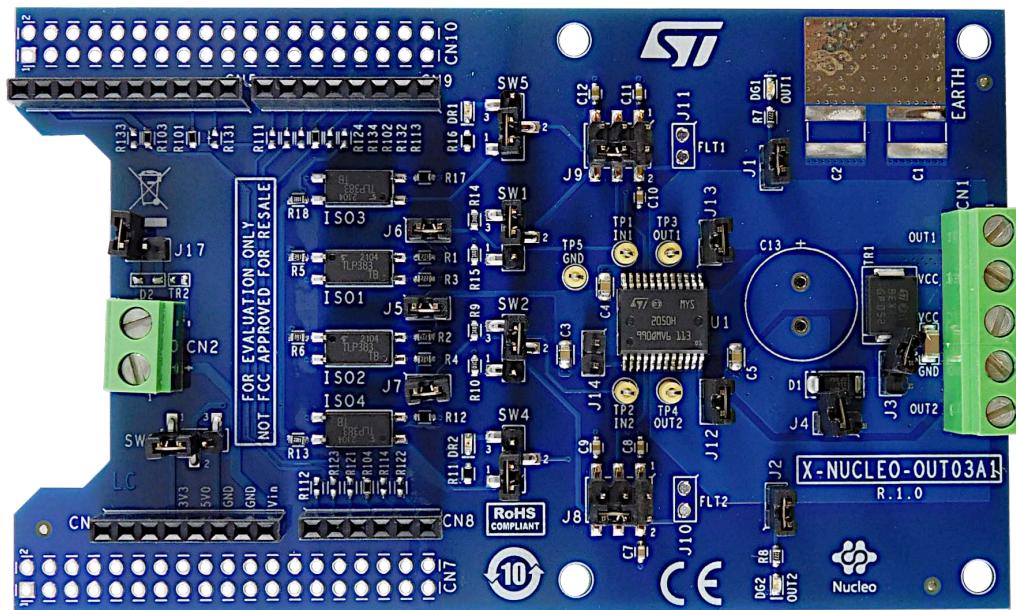
Figure 1. X-NUCLEO-OUT03A1 expansion board
