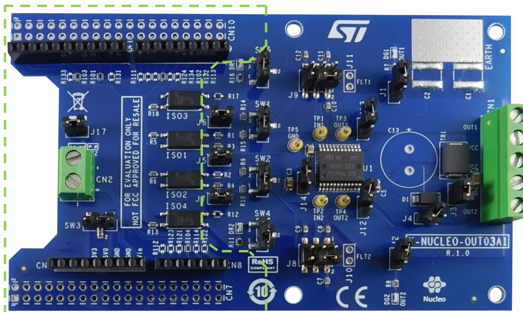
Figure 2. X-NUCLEO-OUT03A1 expansion board: digital interface components
