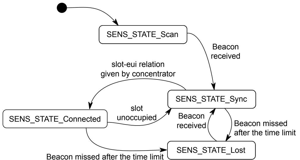
Figure 2. Sensor state diagram
