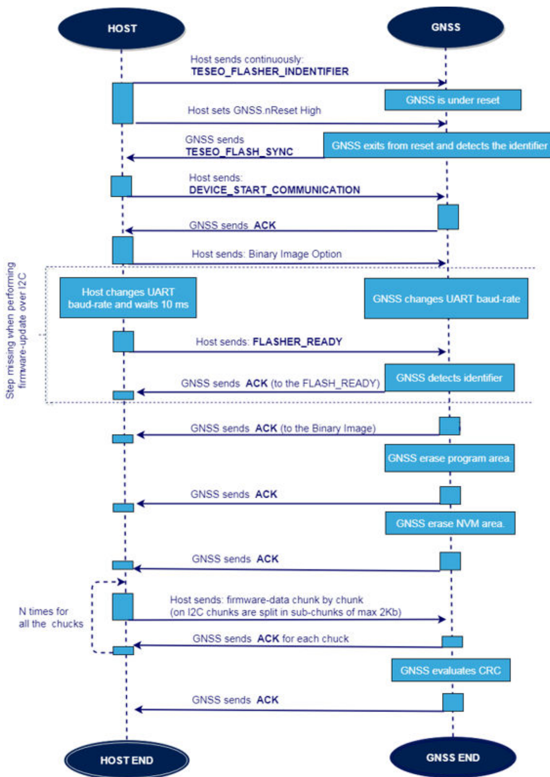
Figure 4. Teseo-Module firmware upgrade procedure on reset
