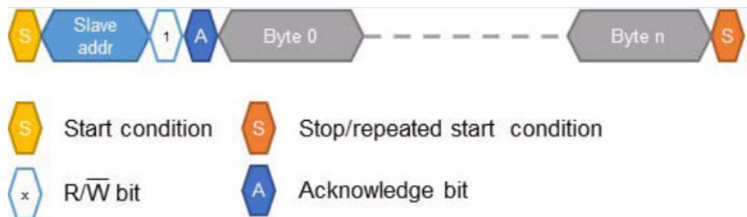
Figure 6. Read operation description
