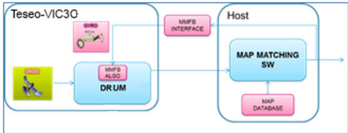
Figure 11. Navigation system feat. MMFB on Teseo-VIC30
