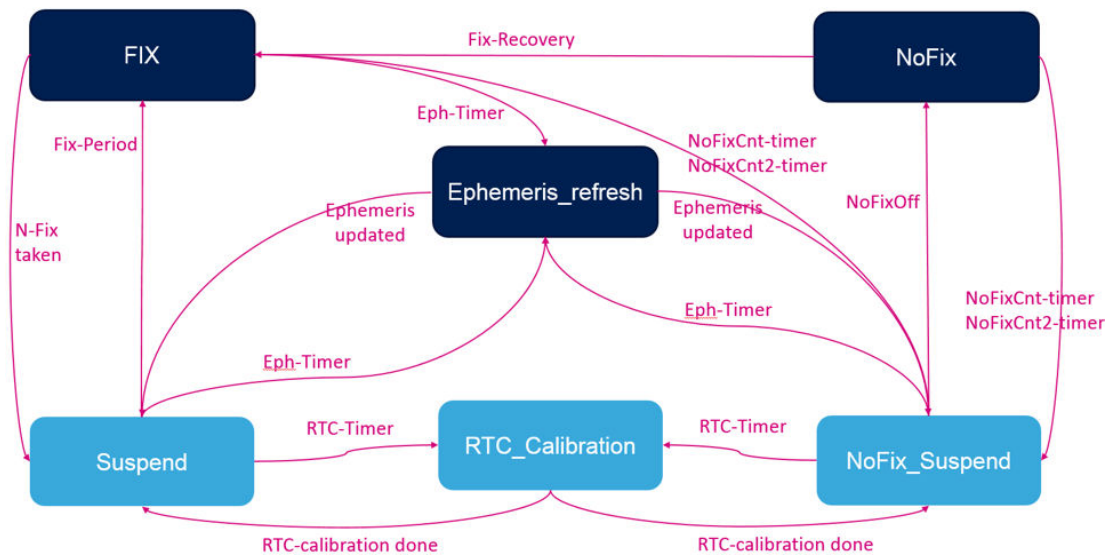
Figure 18. Low power periodic mode state diagram
