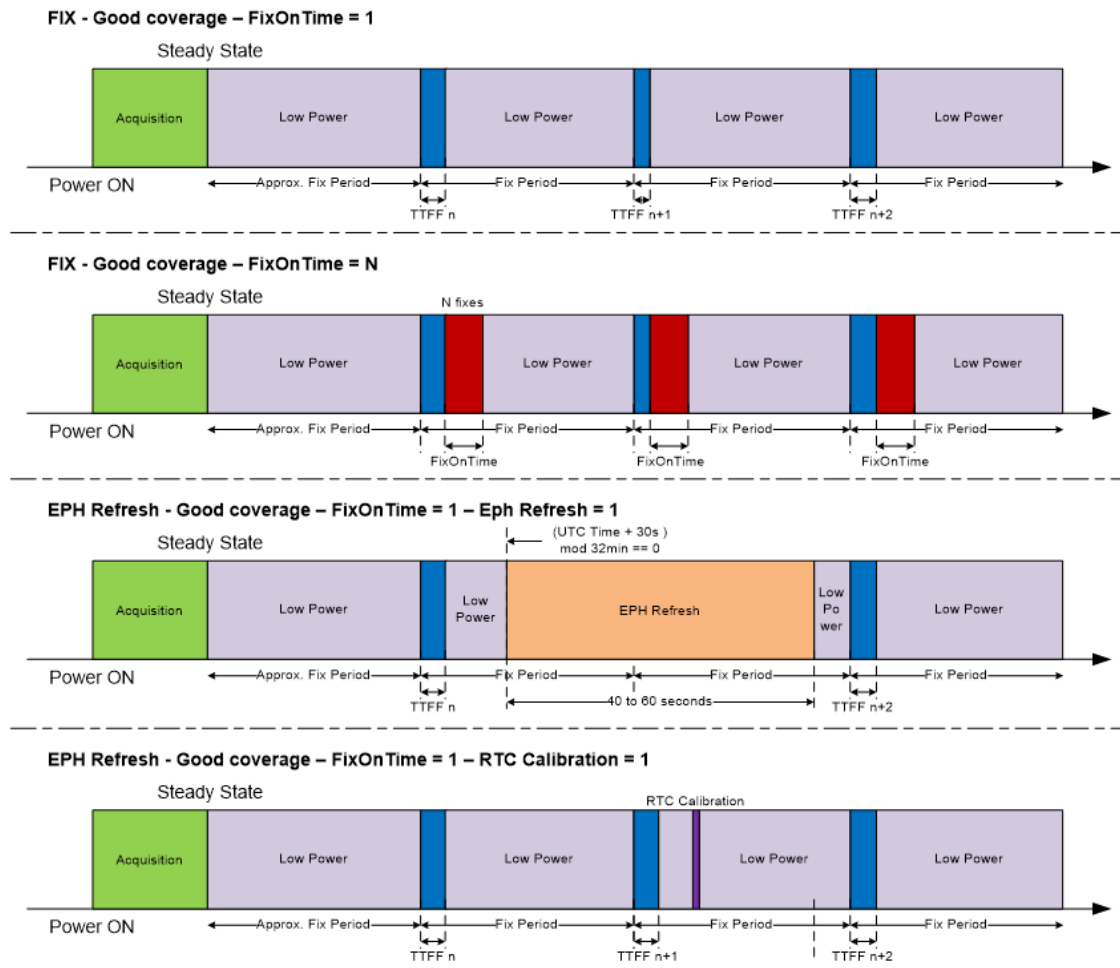
Figure 19. GNSS good coverage sequences
