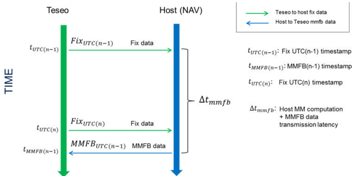
Figure 15. Usage of MMFB interface with incorrect timing
