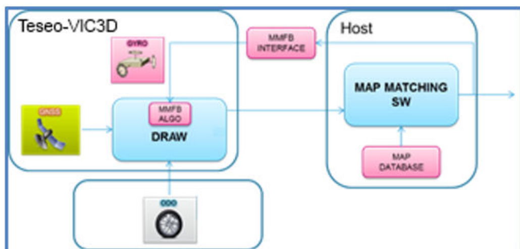
Figure 10. Navigation system feat. MMFB on Teseo-Module
