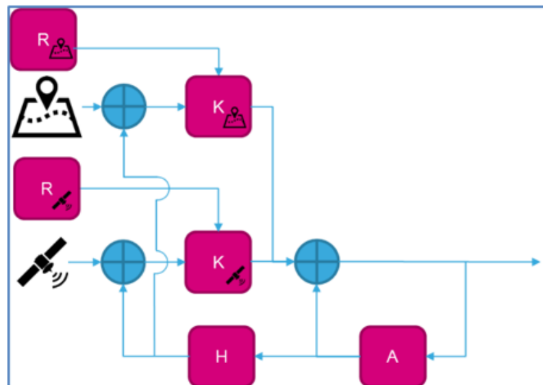
Figure 12. MMFB fusion engine
