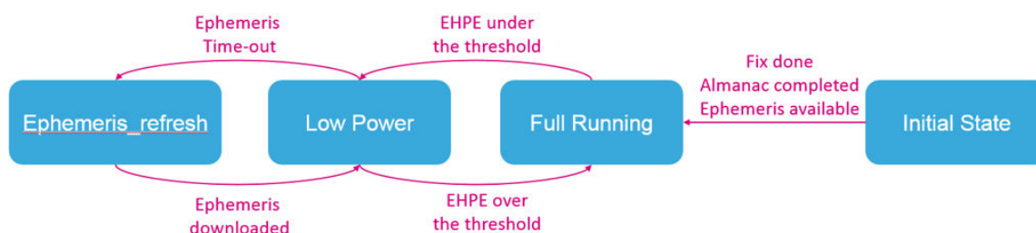
Figure 17. Adaptive and cyclic mode state diagram
