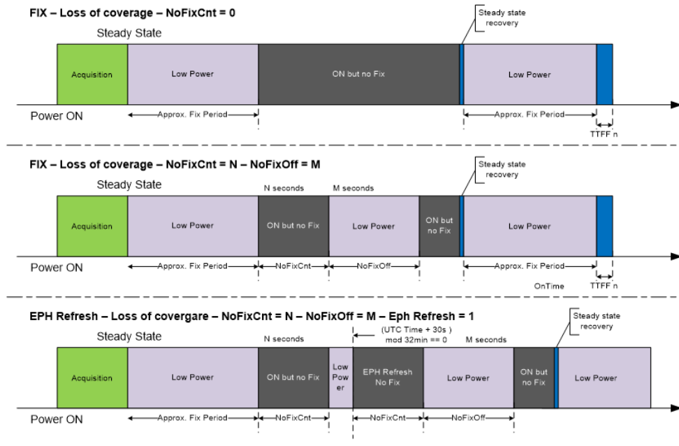
Figure 20. GNSS poor coverage sequences
