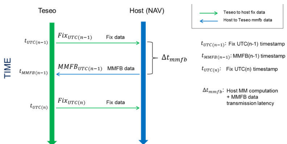
Figure 14. Usage of MMFB interface with correct timing
