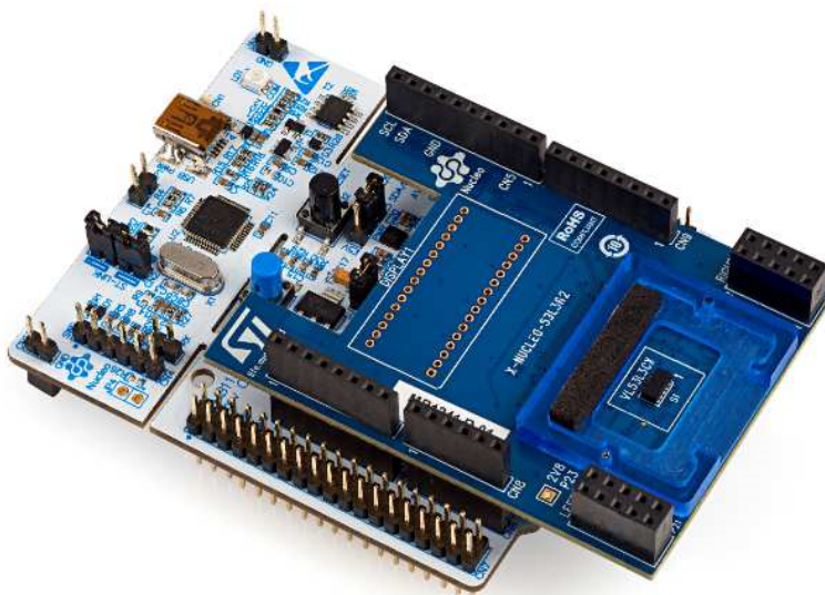
Figure 7. X-NUCLEO-53L3A2 expansion board connected to STM32 Nucleo board
