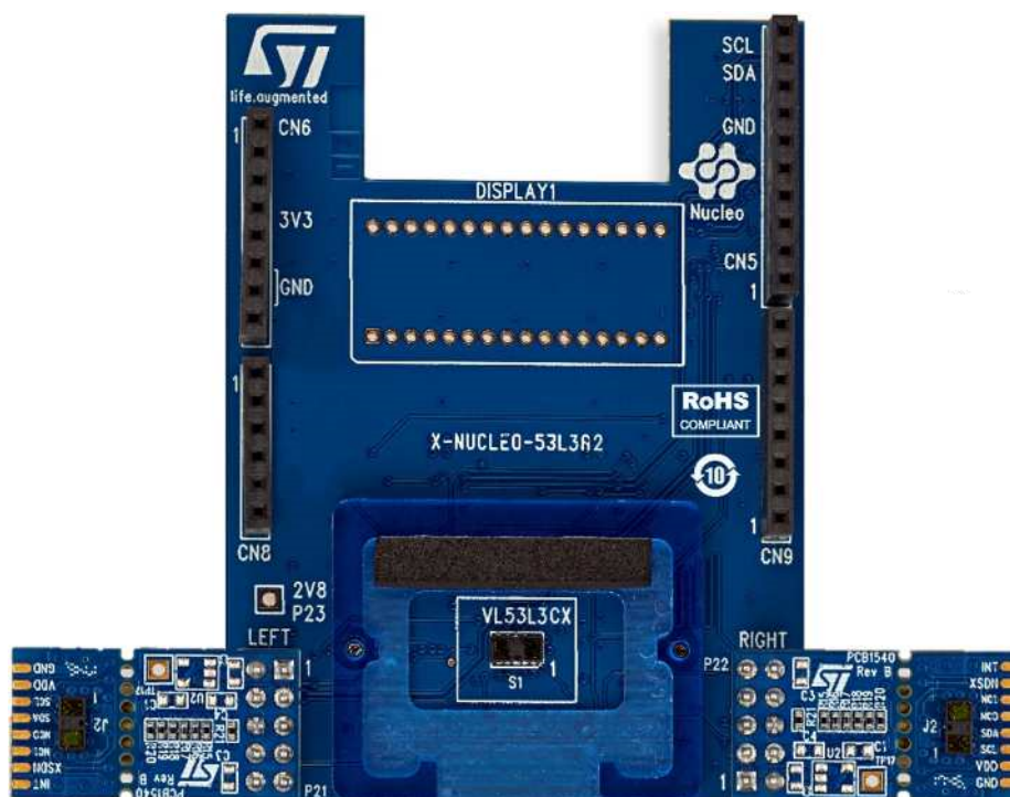
Figure 6. X-Nucleo-53L3A2 expansion board
