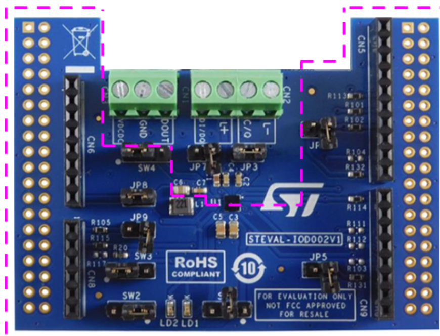
Figure 2. STEVAL-IOD002V1 expansion board digital section
