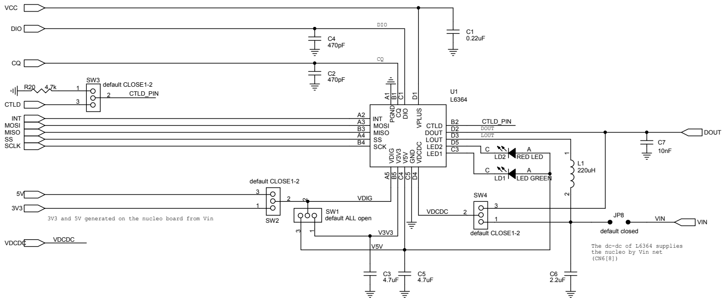
Figure 6. STEVAL-IOD002V1 circuit schematic (2 of 2)
