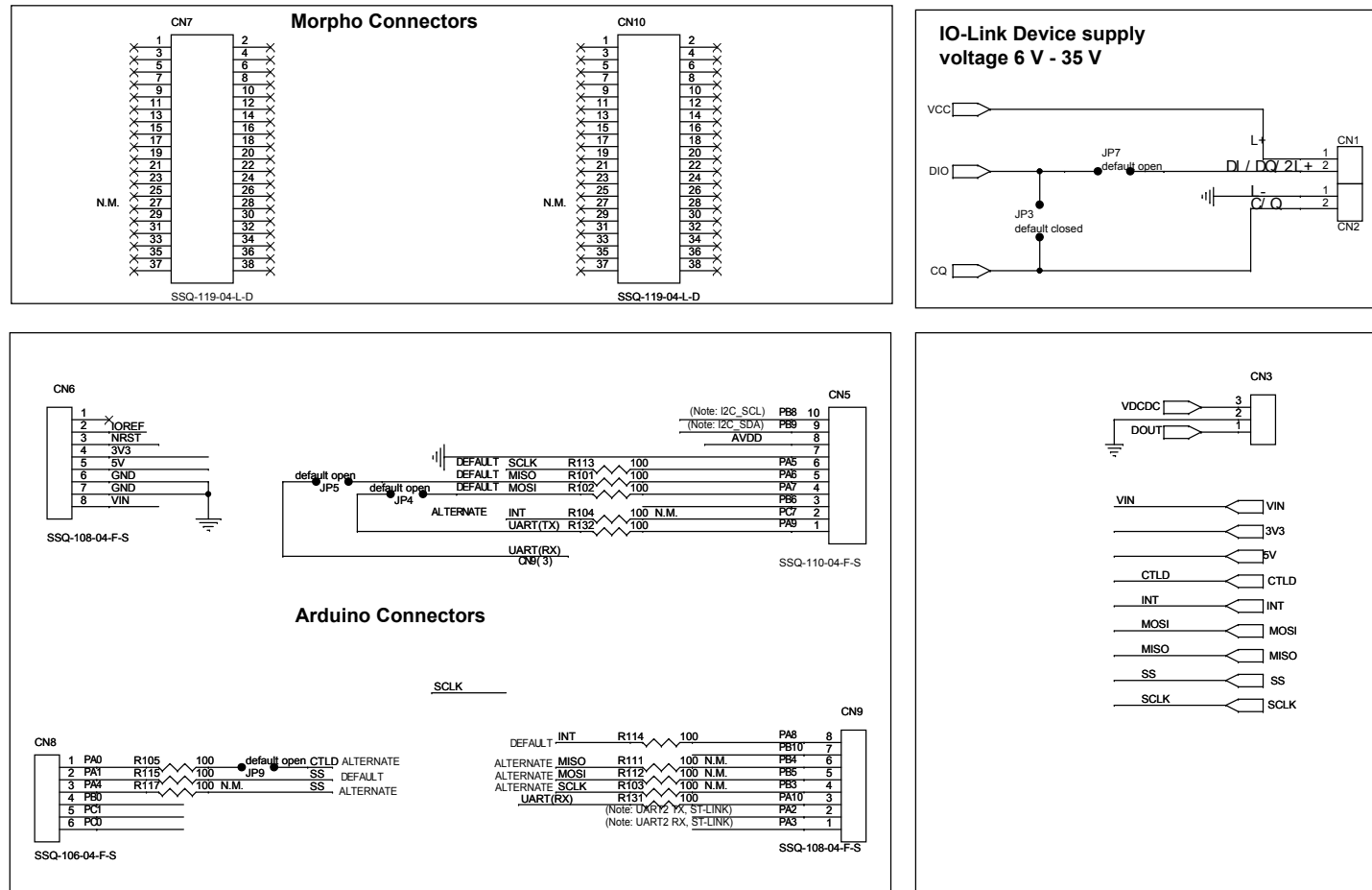
Figure 5. STEVAL-IOD002V1 circuit schematic (1 of 2)
