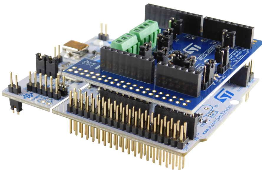
Figure 4. STEVAL-IOD002V1 and STM32 Nucleo stack
