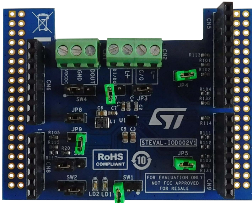
Figure 1. STEVAL-IOD002V1 expansion board
