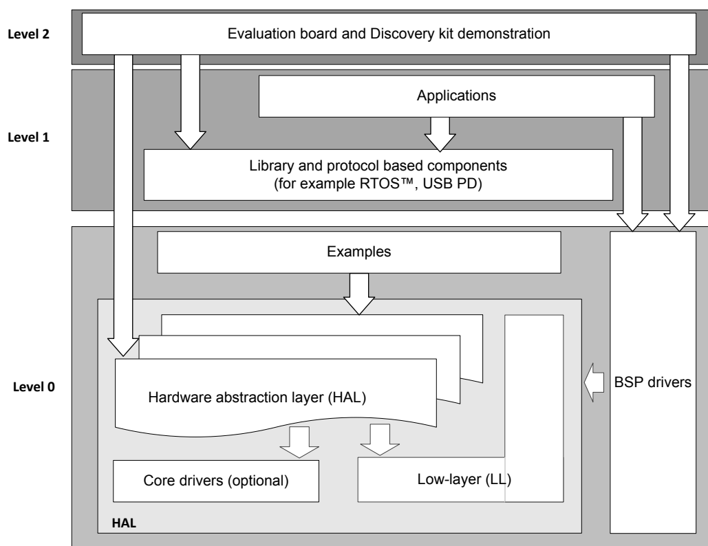
Figure 2. STM32CubeU5 MCU package architecture
