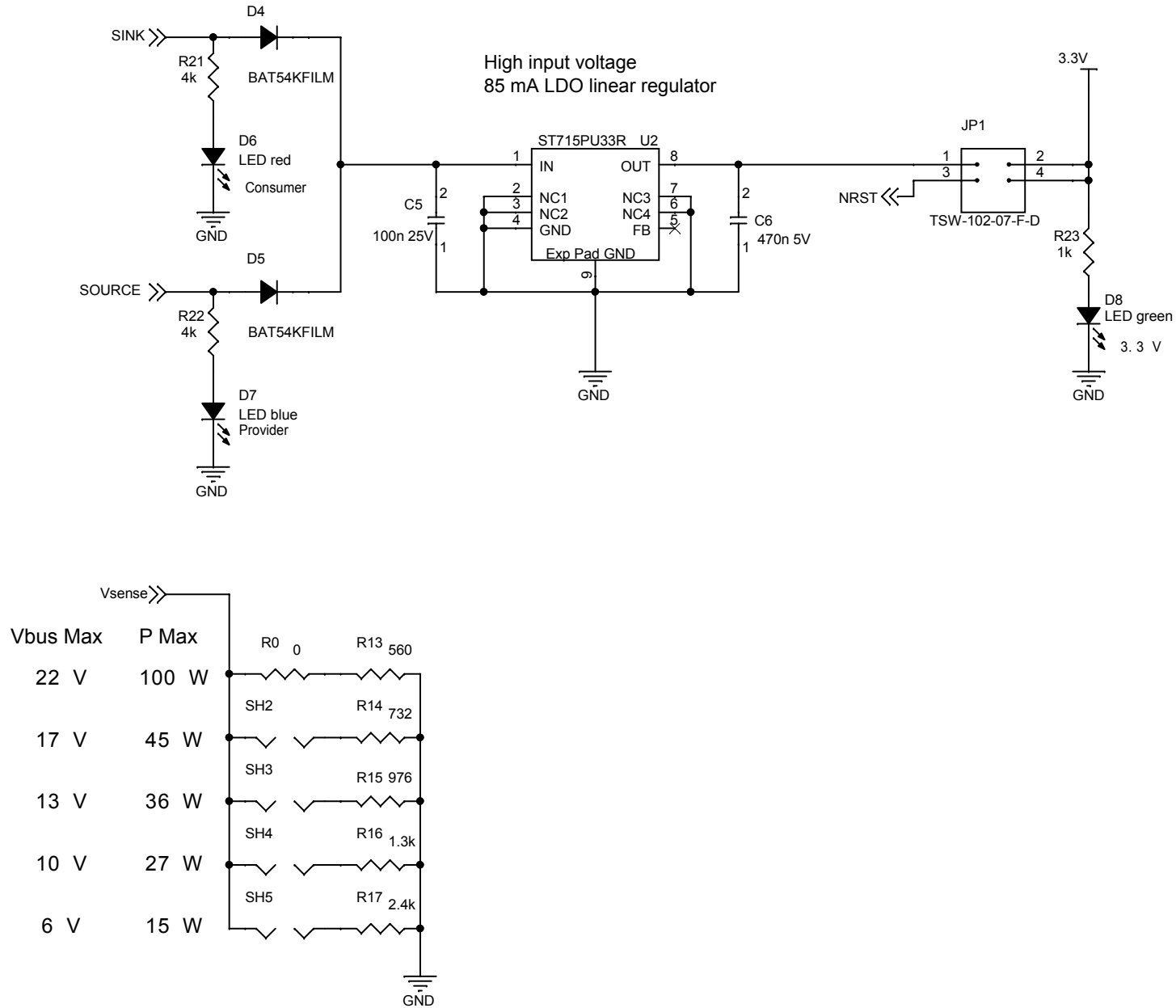
Figure 16. X-NUCLEO-DRP1M1 schematic diagram (3 of 3)
