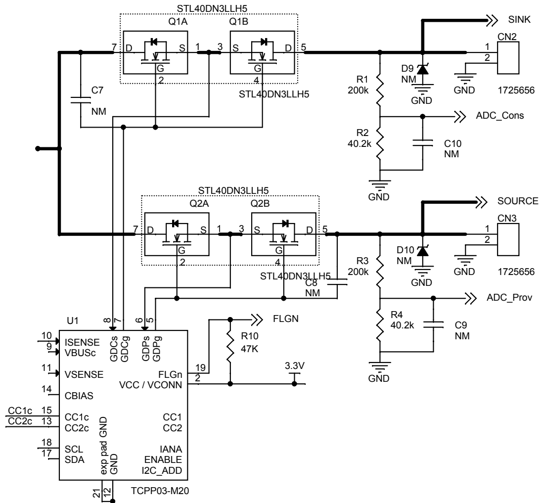
Figure 9. Consumer and provider path
