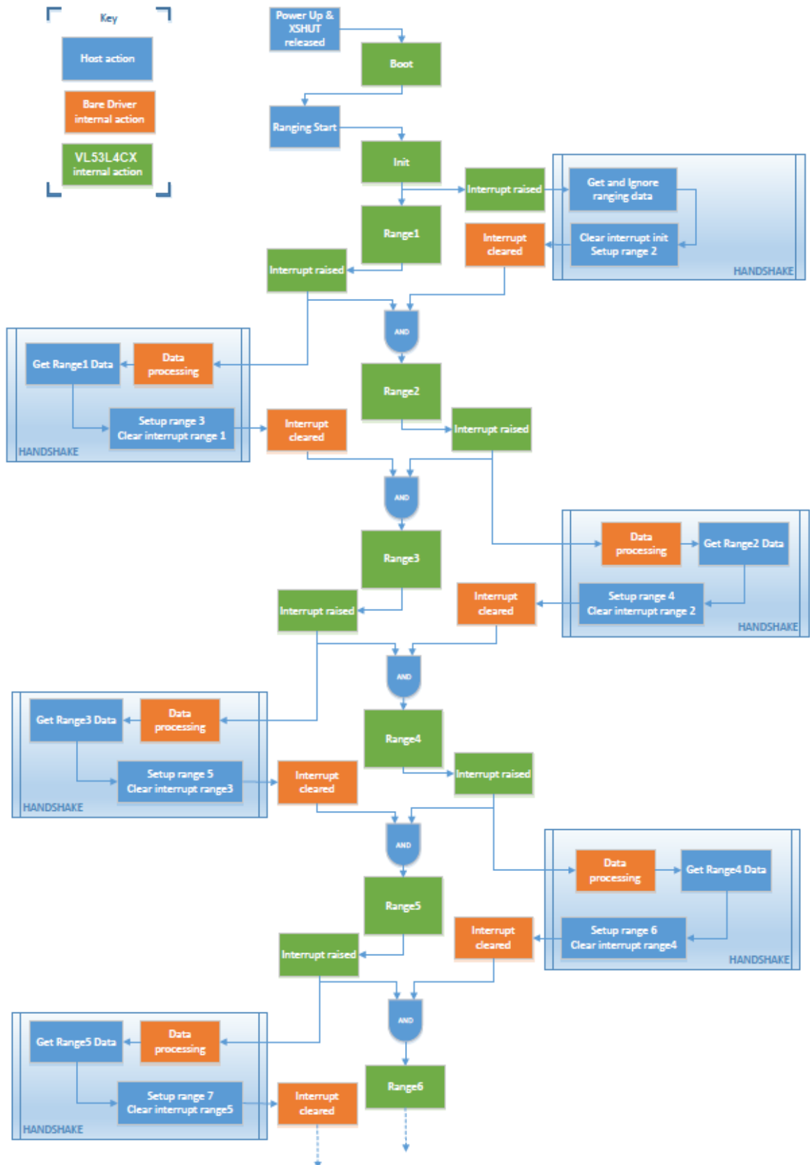
Figure 2. VL53L4CX ranging sequence overview
