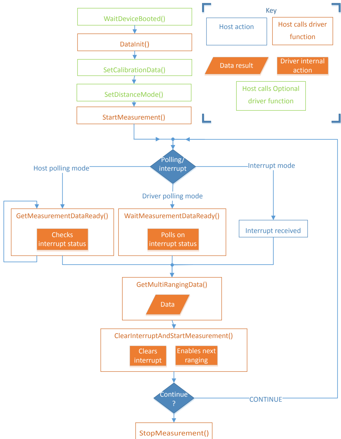
Figure 5. VL53L4CX API ranging flow (field)
