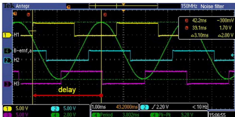
Figure 49. Oscilloscope plot
