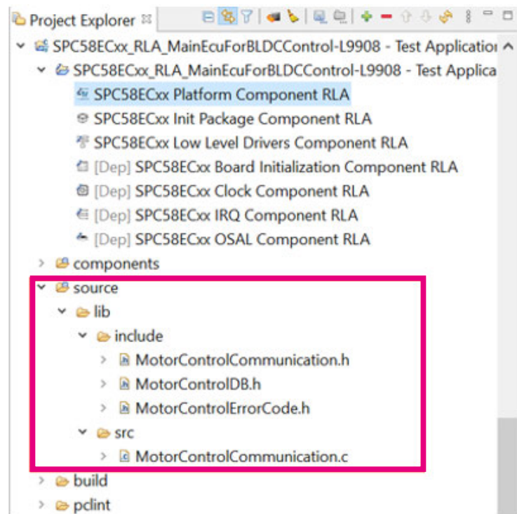
Figure 41. Motor Control Communication library
