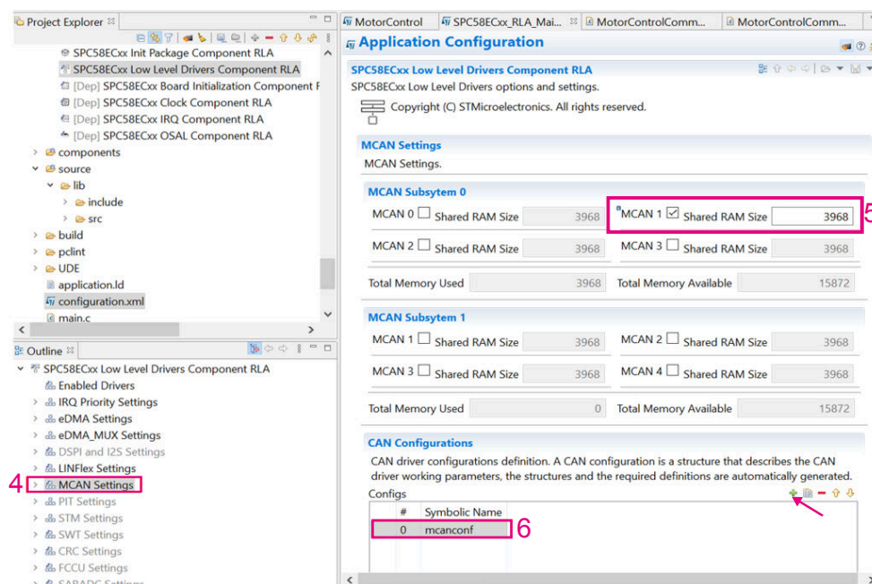
Figure 39. CAN configuration
