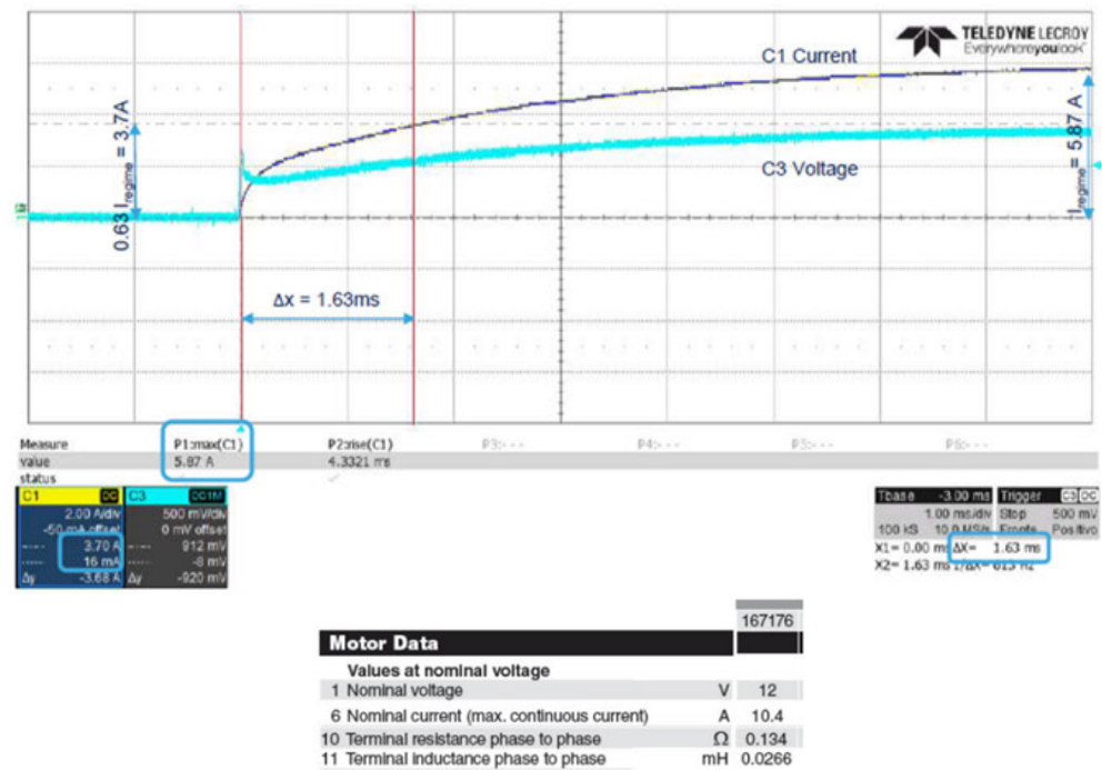
Figure 30. Results of the procedure to determine the stator resistance and inductance of the BLDC motor, when applied to the BLDC motor MAXON EC40
