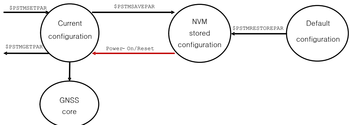
Figure 4. Custom Configuration using NMEA Protocol
