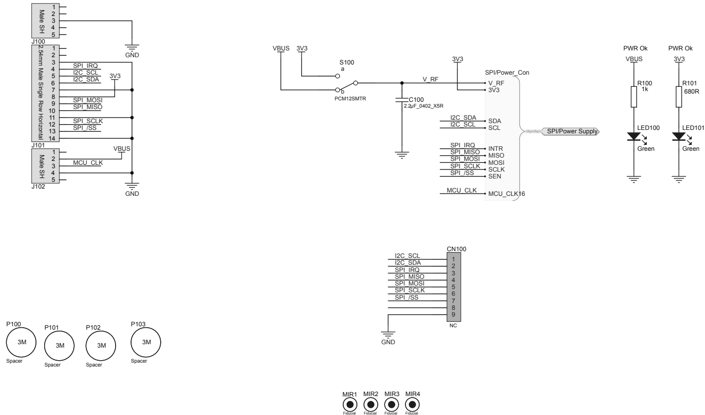
Figure 20. STEVAL-ST25R3916B reader expansion board circuit schematic (1 of 3)
