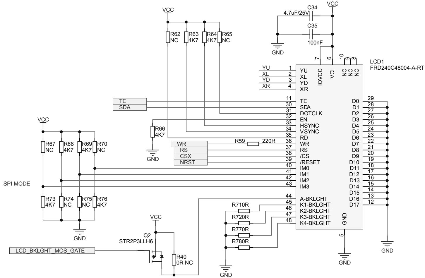
Figure 15. STEVAL-ST25R3916B main board circuit schematic (6 of 10)
