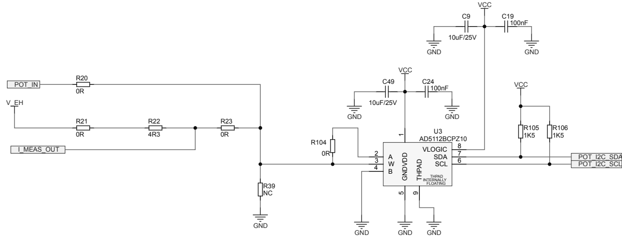
Figure 13. STEVAL-ST25R3916B main board circuit schematic (4 of 10)
