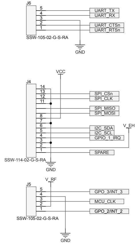
Figure 17. STEVAL-ST25R3916B main board circuit schematic (8 of 10)
