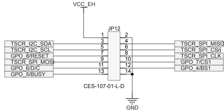
Figure 19. STEVAL-ST25R3916B main board circuit schematic (10 of 10)
