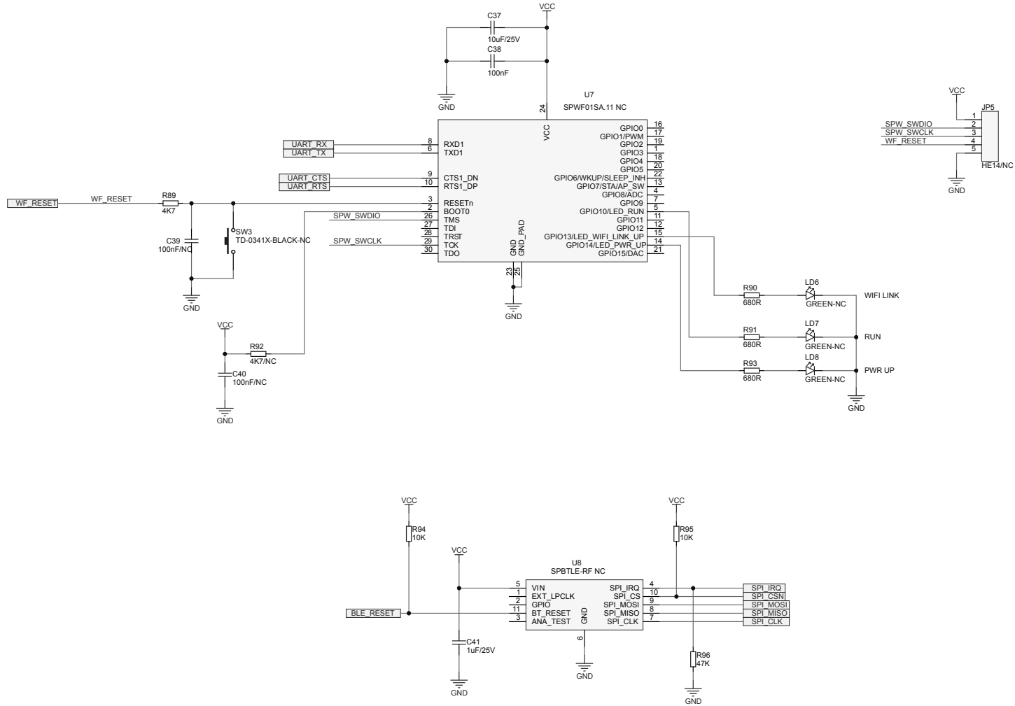
Figure 16. STEVAL-ST25R3916B main board circuit schematic (7 of 10)
