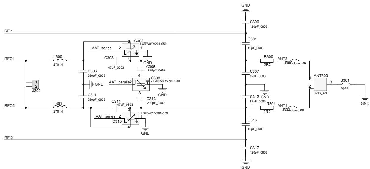
Figure 22. STEVAL-ST25R3916B reader expansion board circuit schematic (3 of 3)
