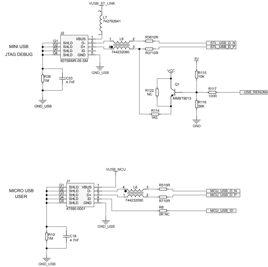
Figure 18. STEVAL-ST25R3916B main board circuit schematic (9 of 10)
