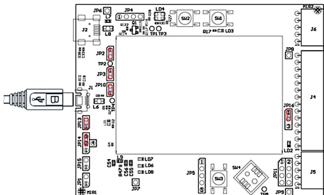
Figure 5. Jumper default configuration
