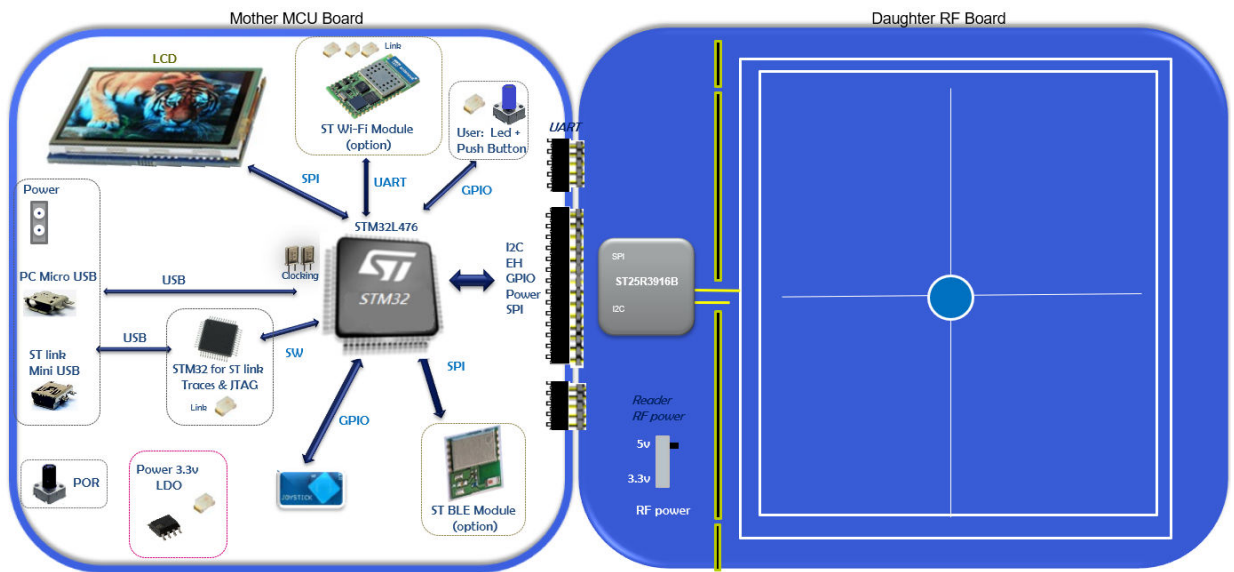
Figure 2. Hardware connection
