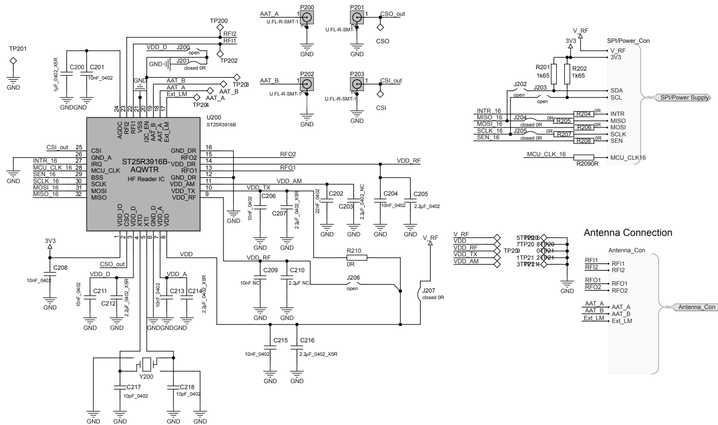
Figure 21. STEVAL-ST25R3916B reader expansion board circuit schematic (2 of 3)
