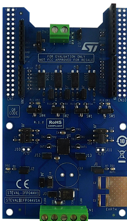
Figure 1. STEVAL-IFP044V1 expansion board
