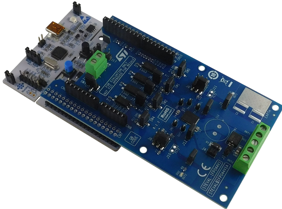
Figure 4. STEVAL-IFP044V1 and STM32 Nucleo stack
