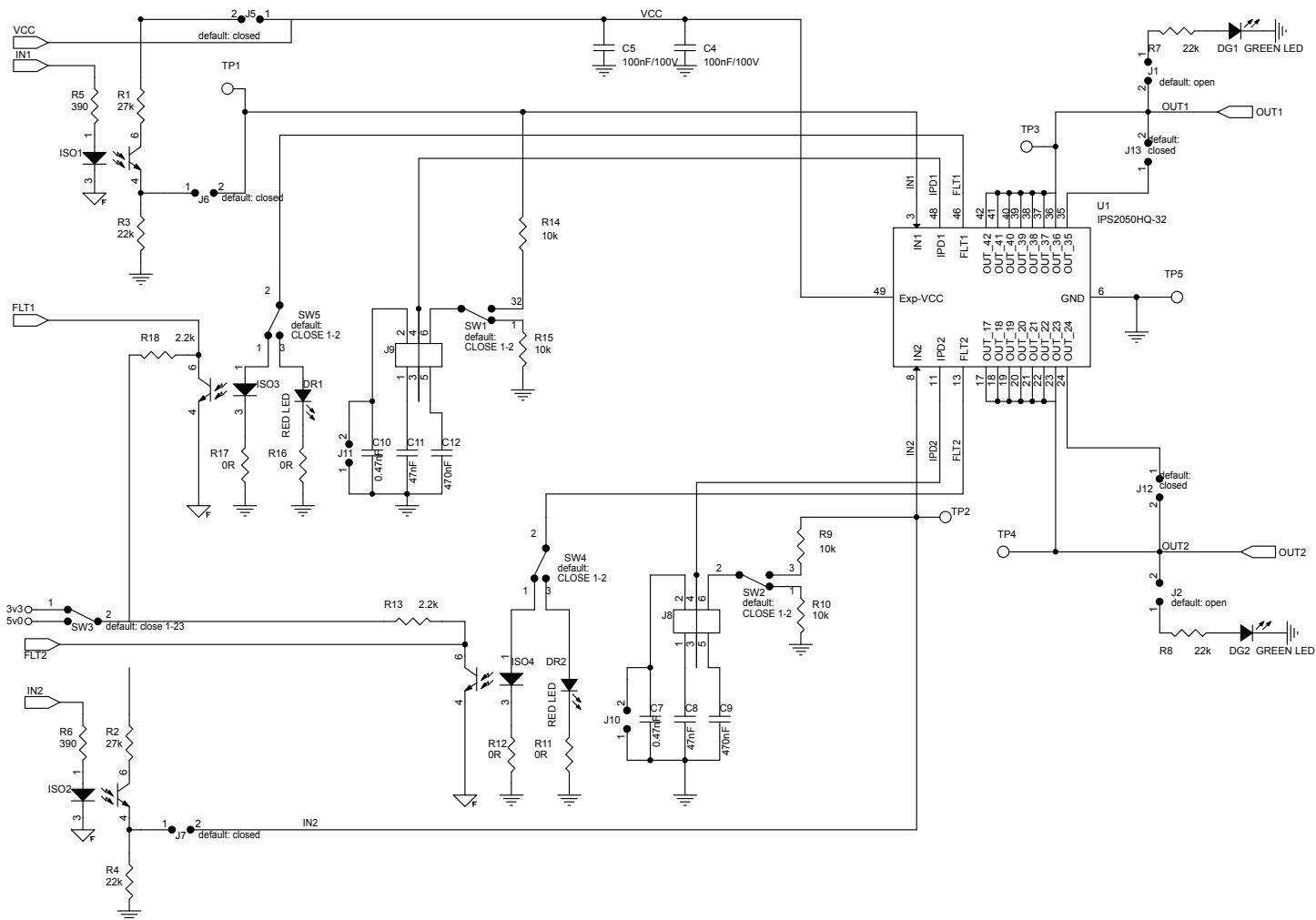
Figure 6. STEVAL-IFP044V1 circuit schematic (2 of 2)
