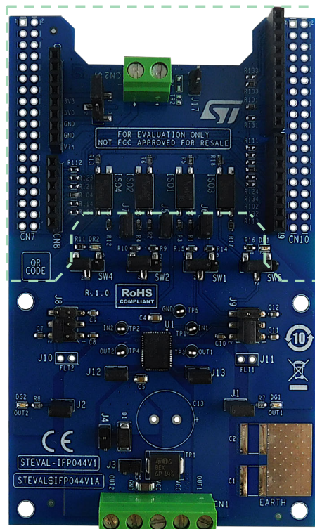
Figure 2. STEVAL-IFP044V1 expansion board: digital interface components
