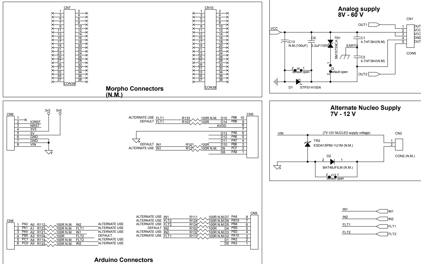
Figure 5. STEVAL-IFP044V1 circuit schematic (1 of 2)
