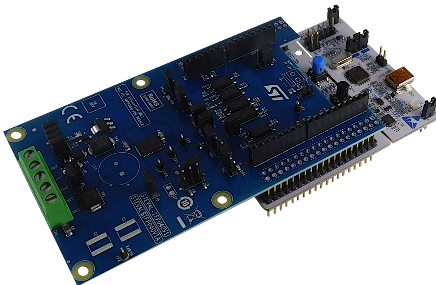
Figure 4. STEVAL-IFP040V1 and STM32 Nucleo stack
