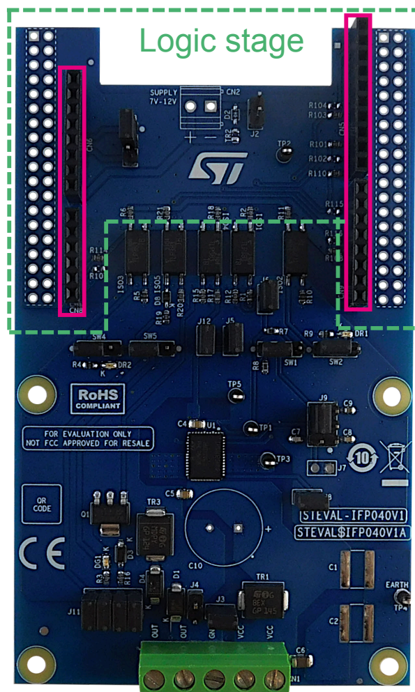
Figure 2. STEVAL-IFP040V1 expansion board: digital interface section
