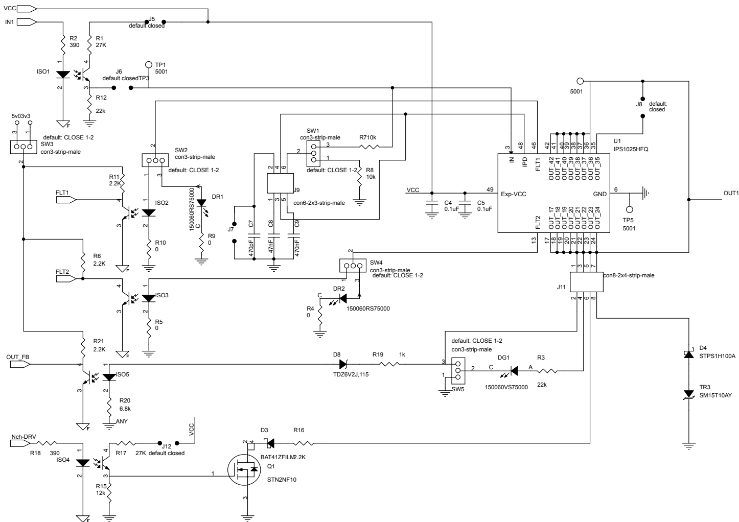
Figure 6. STEVAL-IFP040V1 circuit schematic (2 of 2)
