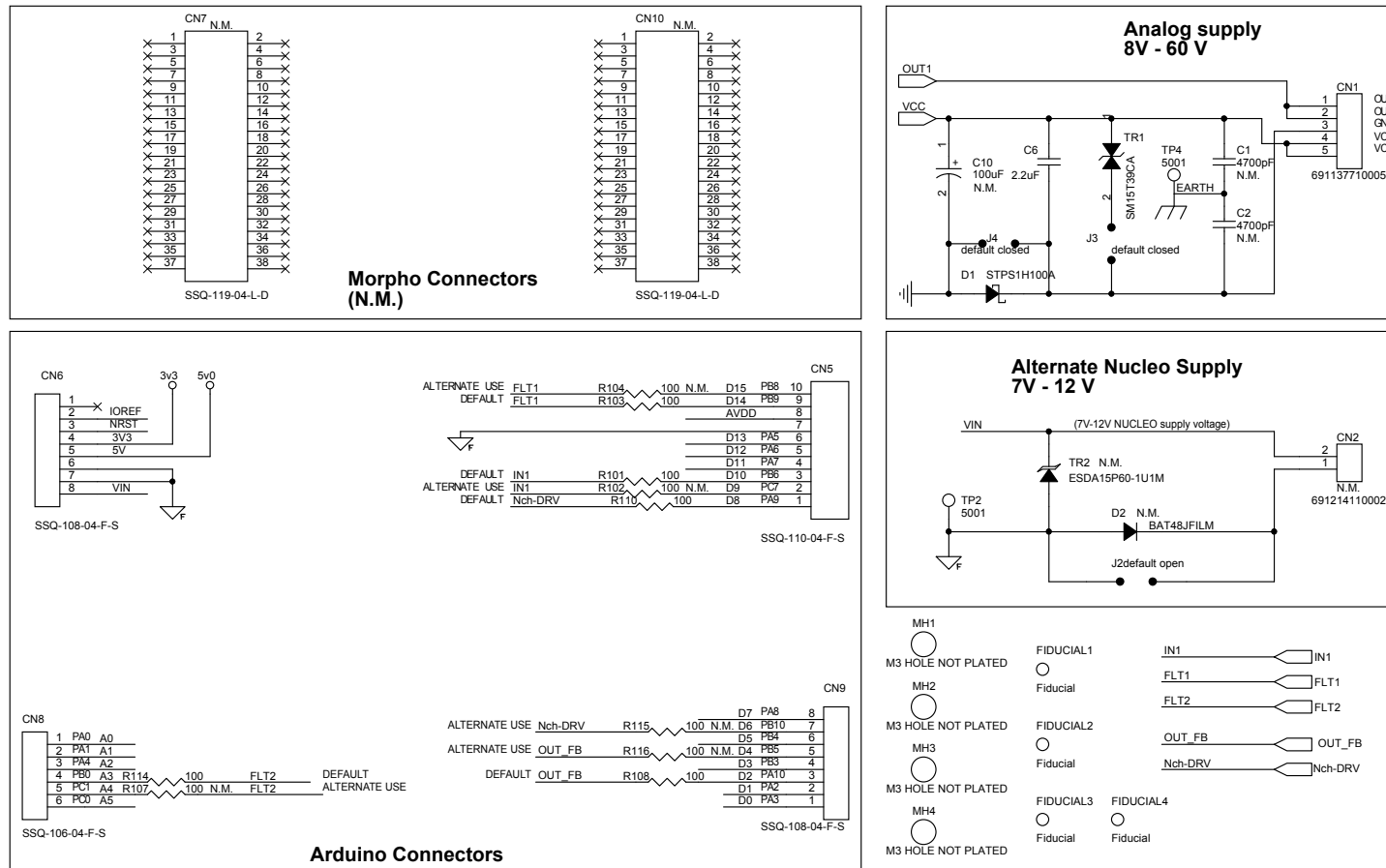
Figure 5. STEVAL-IFP040V1 circuit schematic (1 of 2)
