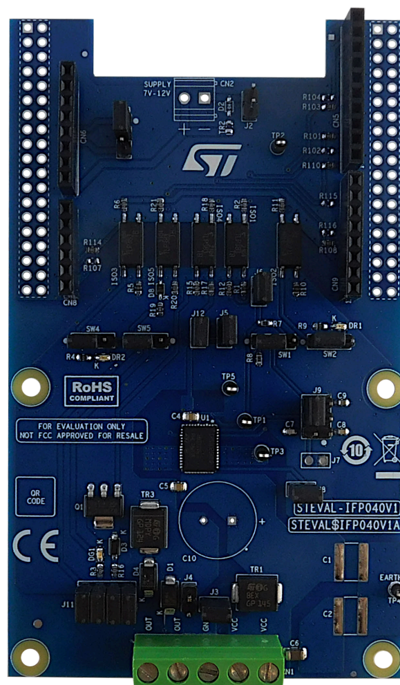
Figure 1. STEVAL-IFP040V1 expansion board
