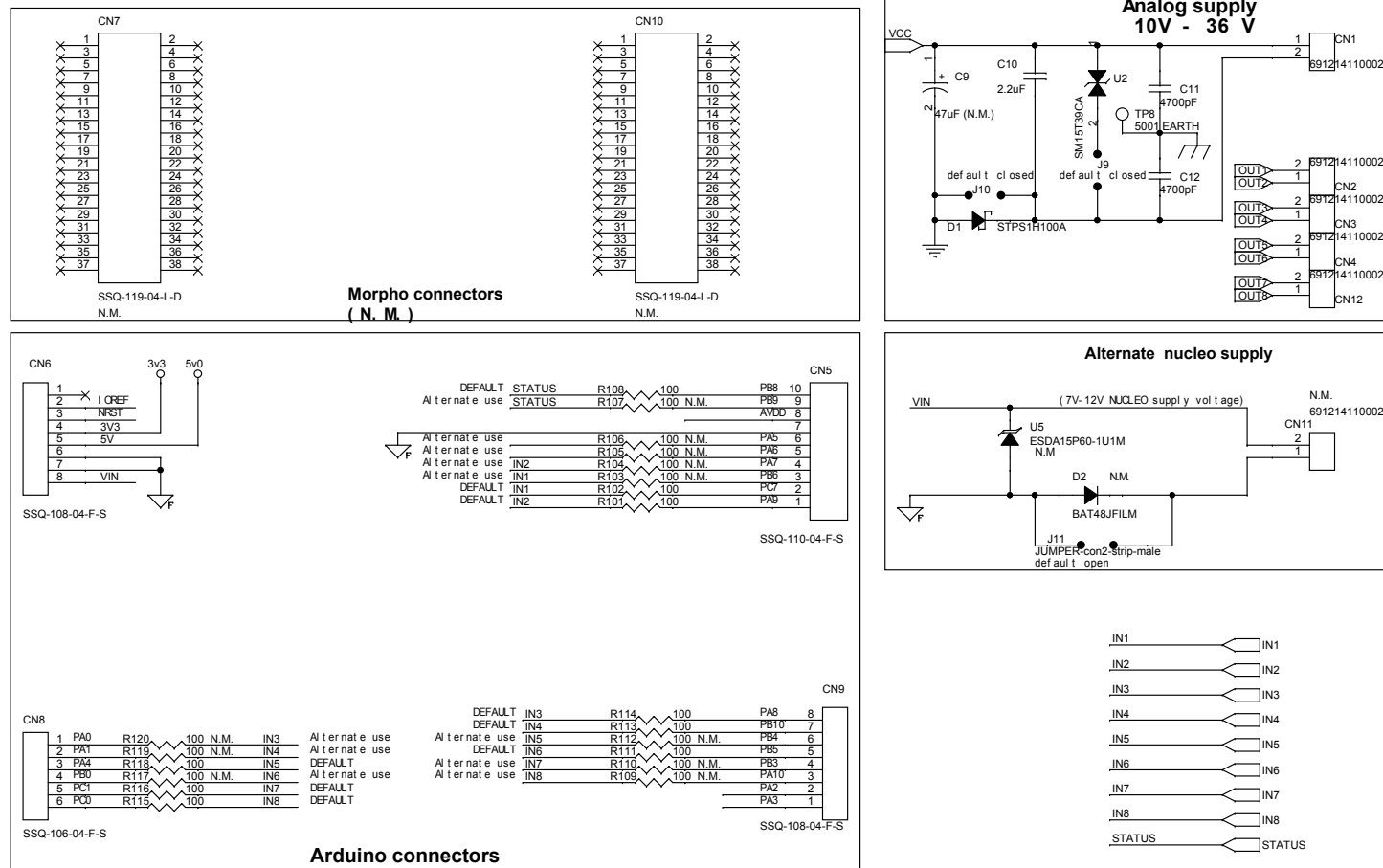
Figure 5. X-NUCLEO-OUT19A1 circuit schematic (1 of 2)
