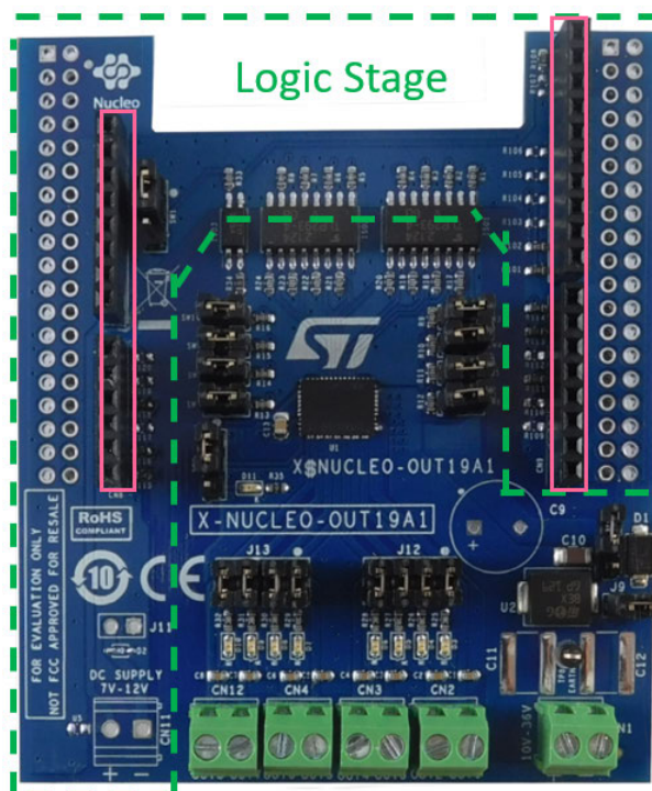
Figure 2. X-NUCLEO-OUT19A1 expansion board: digital interface section
