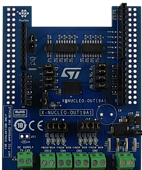
Figure 1. X-NUCLEO-OUT19A1 expansion board
