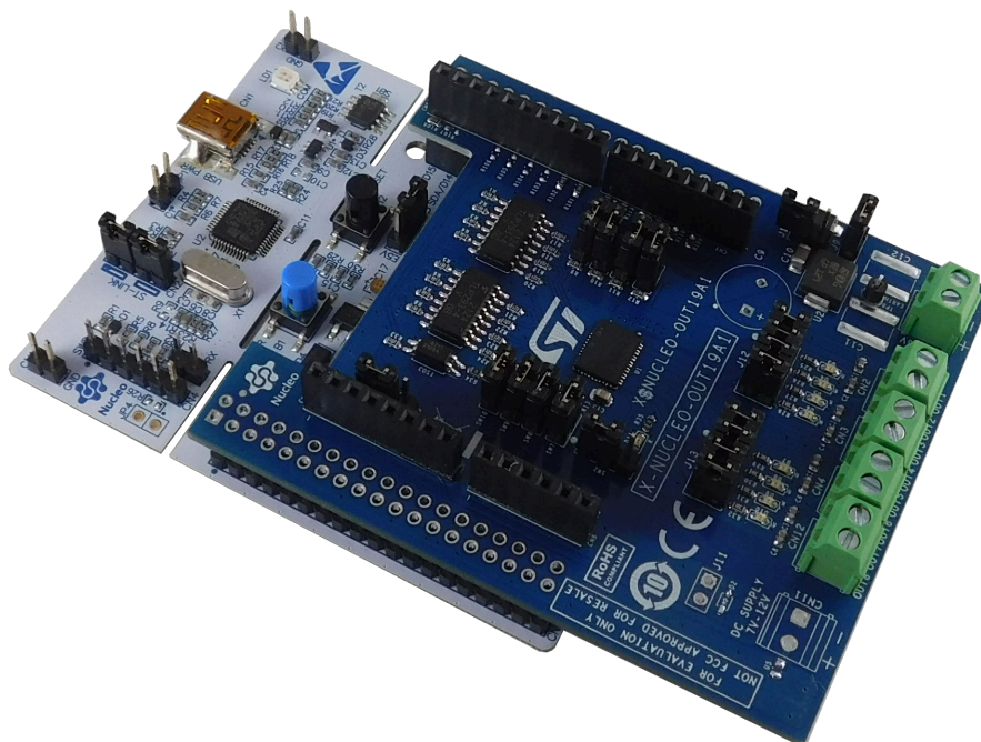
Figure 4. X-NUCLEO-OUT19A1 and STM32 Nucleo stack
