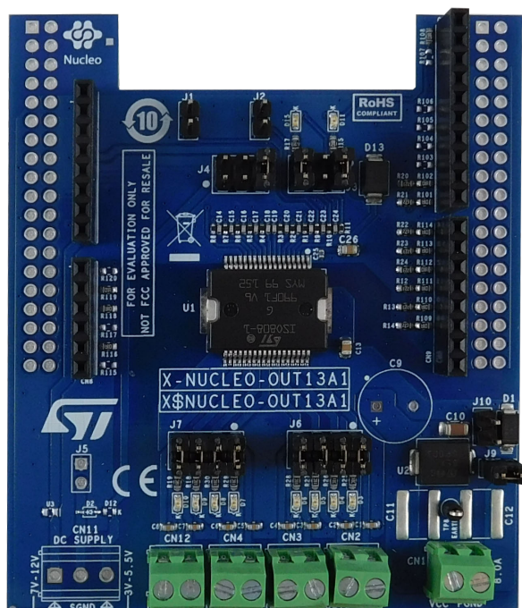
Figure 1. X-NUCLEO-OUT13A1 expansion board
