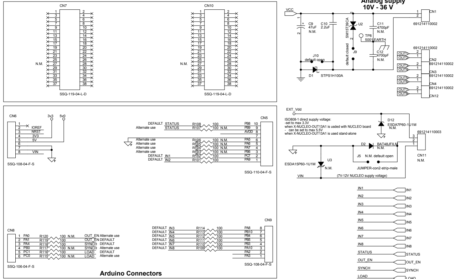
Figure 5. X-NUCLEO-OUT13A1 circuit schematic (1 of 2)
