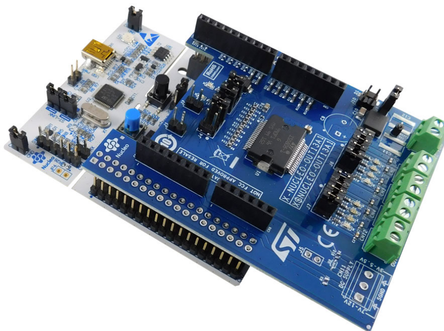
Figure 4. X-NUCLEO-OUT13A1 and STM32 Nucleo stack
