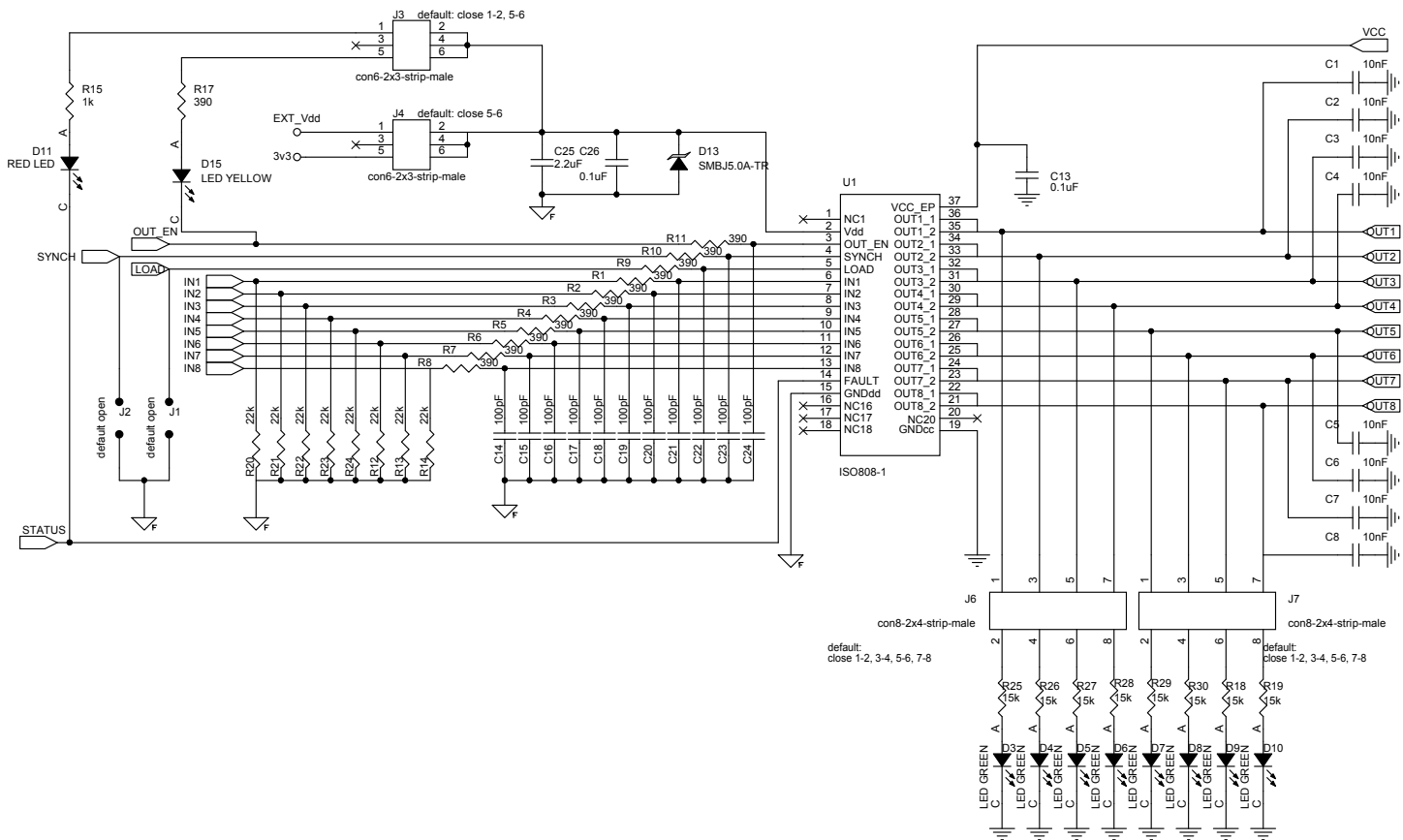
Figure 6. X-NUCLEO-OUT13A1 circuit schematic (2 of 2)
