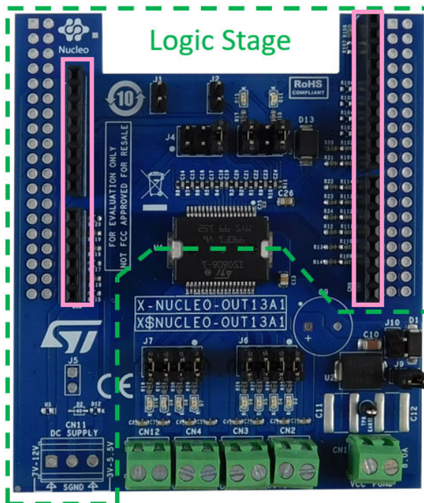
Figure 2. X-NUCLEO-OUT13A1 expansion board: digital interface section
