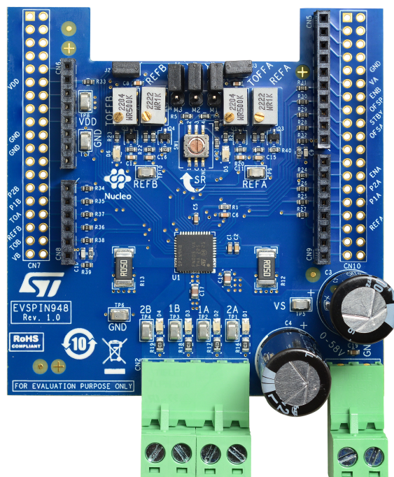
Figure 1. EVSPIN948 evaluation board
