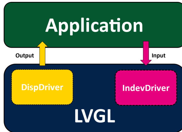
Figure 2. LVGL drivers
