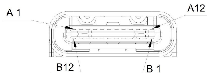
Figure 22. STLINK-V3EC connector (CN7) front view
