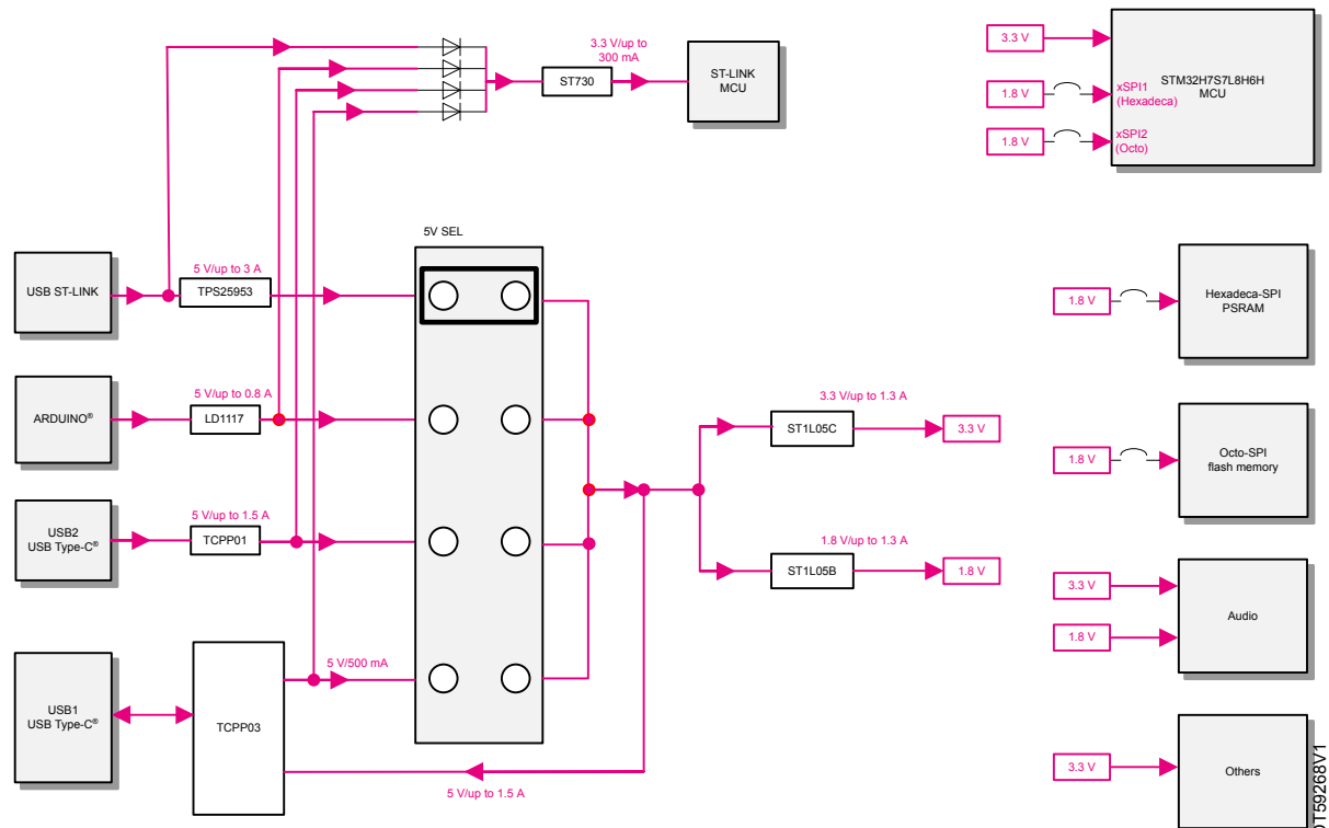
Figure 7. Power diagram
