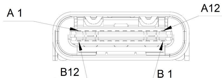
Figure 27. User USB2 Type-C connector (CN17) front view
