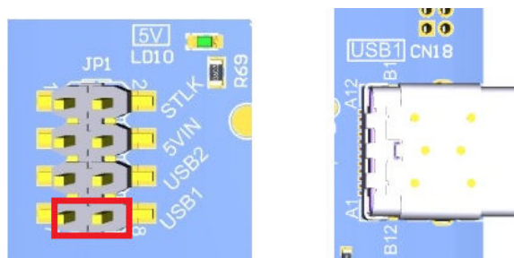
Figure 11. JP1 (USB1) from CN18 (USB1 Type-C)
