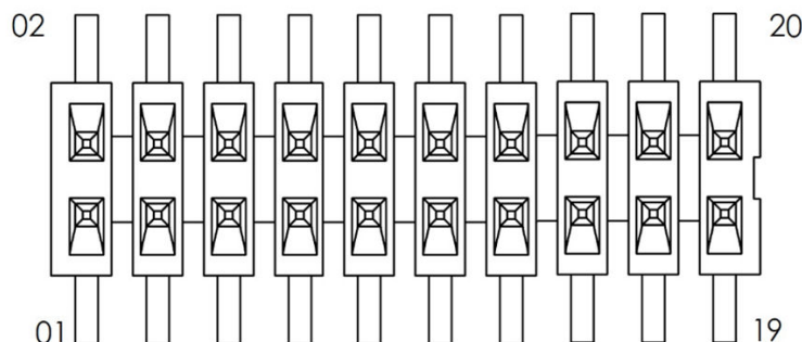
Figure 23. MIPI20 debug connector (CN8) top view
