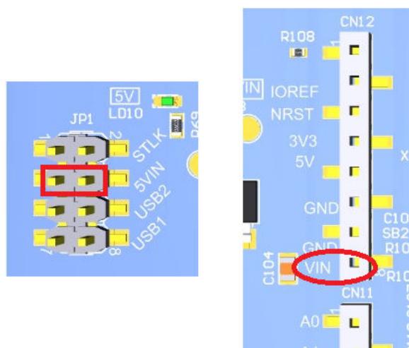
Figure 9. JP1 (5VIN) from CN12 (VIN)
