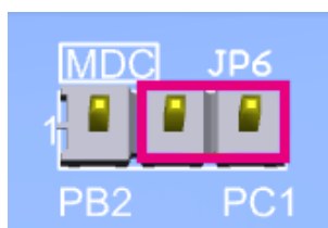
Figure 13. JP6 (MDC) set to PC1
