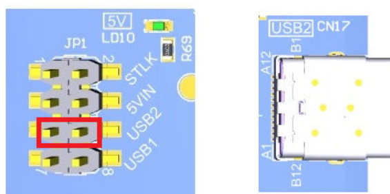
Figure 10. JP1 (USB2) from CN17 (USB2 Type-C)
