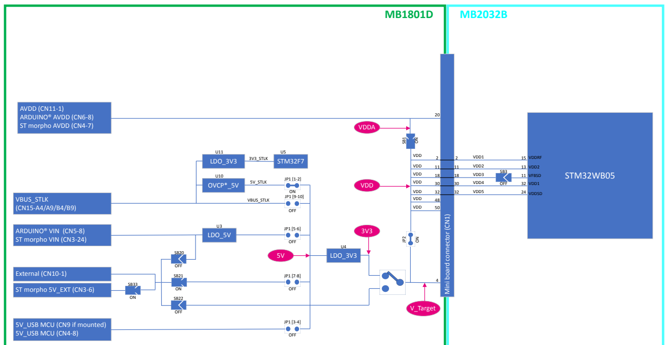
Figure 7. STM32WB05KZ power tree
