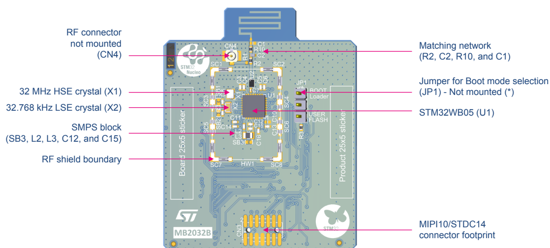
Figure 4. NUCLEO-WB05KZ PCB details of the MCU RF board
