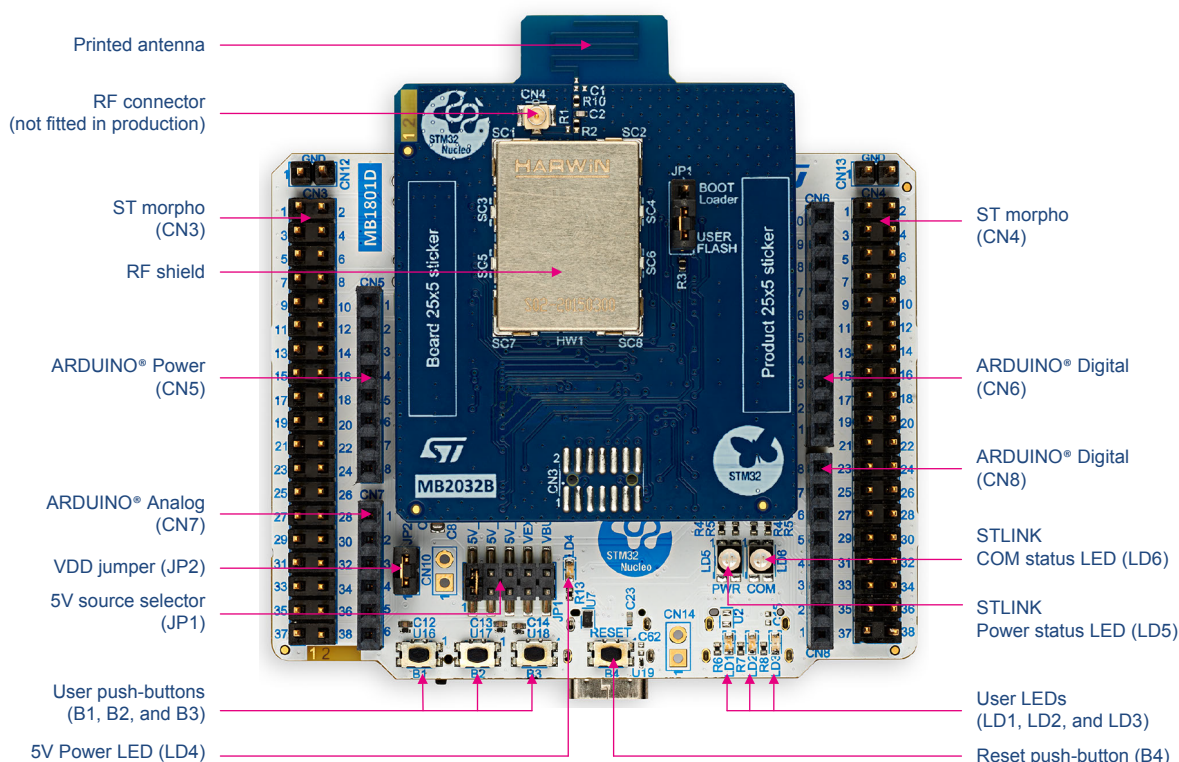
Figure 3. NUCLEO-WB05KZ PCB top view
