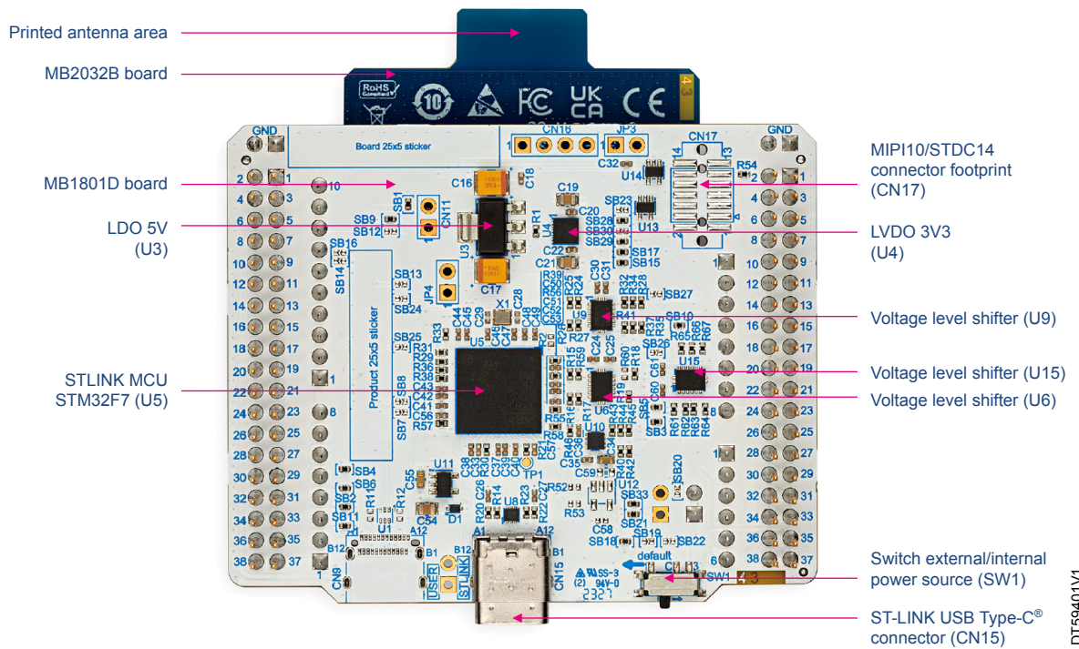
Figure 5. NUCLEO-WB05KZ PCB bottom view
