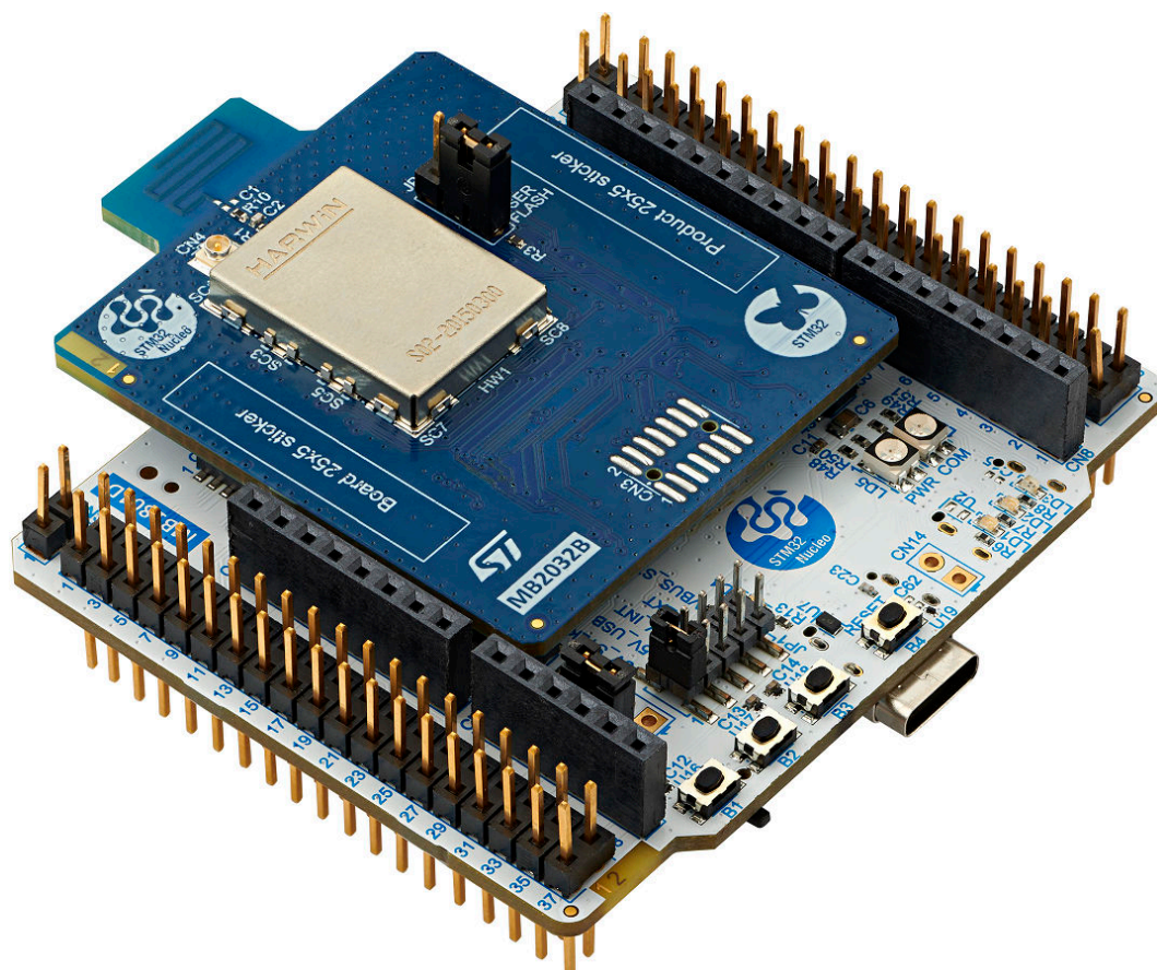
Figure 1. NUCLEO-WB05KZ global view
