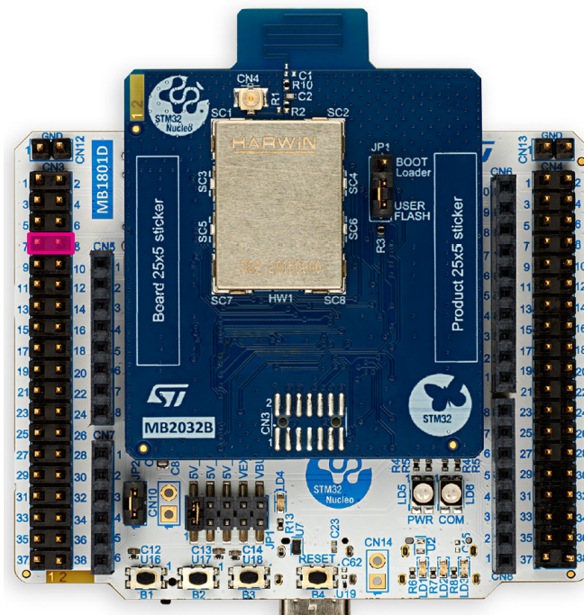
Figure 17. JP3 (MB1801 board) default setting
