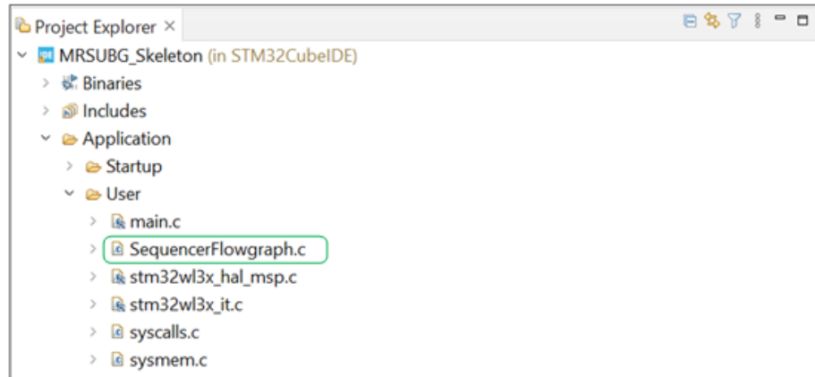
Figure 11. STM32CubeIDE project
