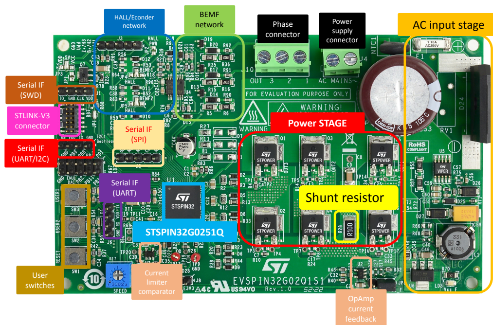
Figure 2. Board function blocks
