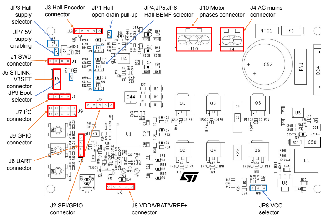
Figure 3. Main components and connector positions
