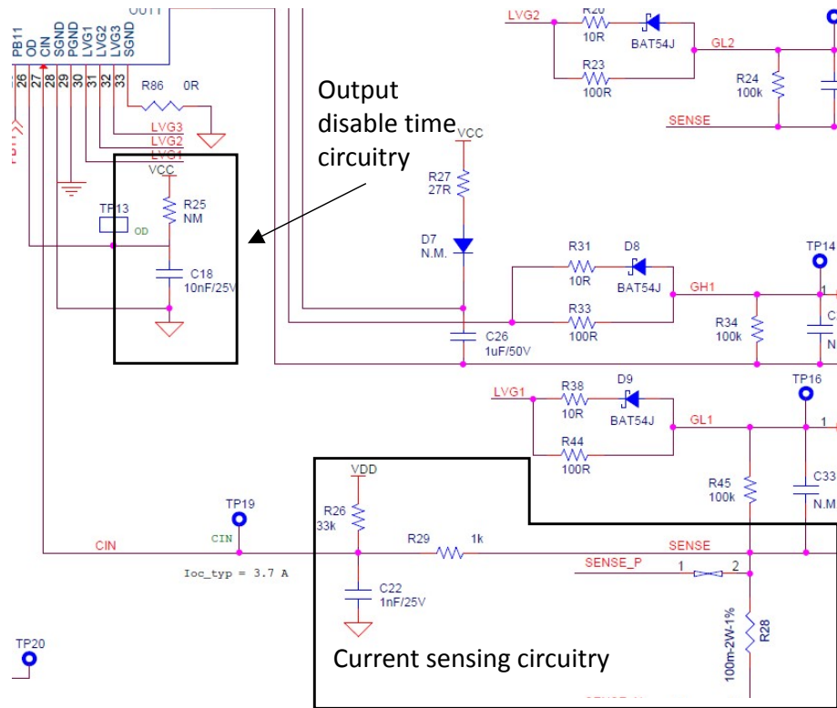
Figure 4. Current sensing and disable time circuitry
