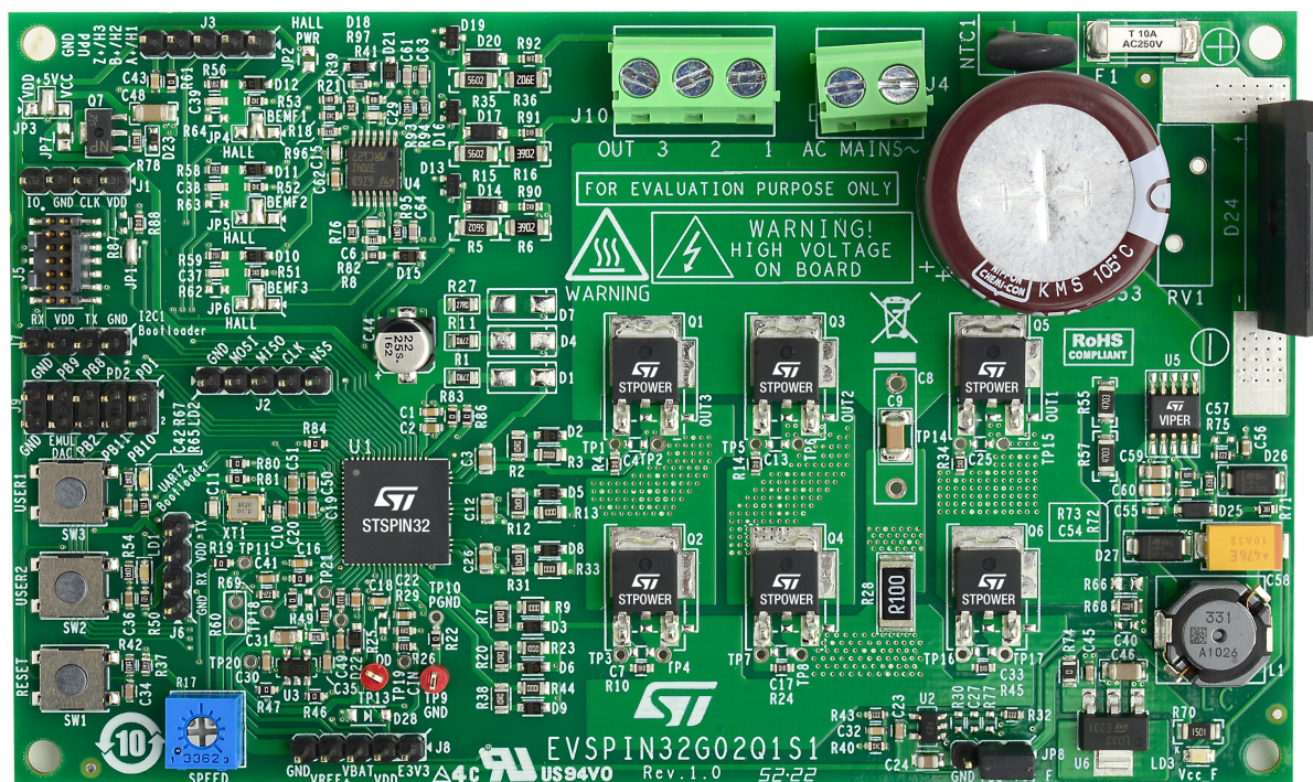
Figure 1. EVSPIN32G02Q1S1 evaluation board
